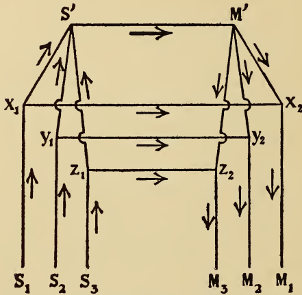
FIG. 7. — DIAGRAM OF NERVOUS ARCHITECTURE: REFLEX ARCHES CONNECTED BY A LOW NERVE CENTER.
