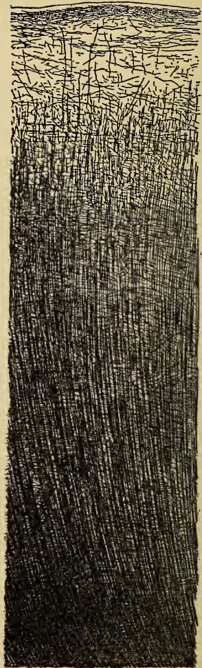
FIG. 12.—SECTION OF THE CEREBRAL CORTEX.
