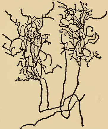
FIG. 6.—TERMINAL ARBORIZATION OF OPTICAL NERVE FIBERS.
