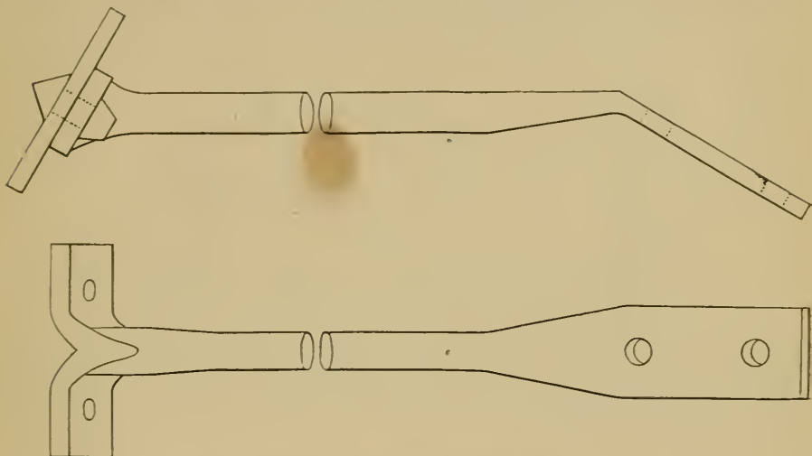
FIG. 9. — CROW-FOOT BRACES.
