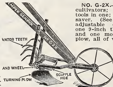
No. G-2X—Single Wheel Cultivator
