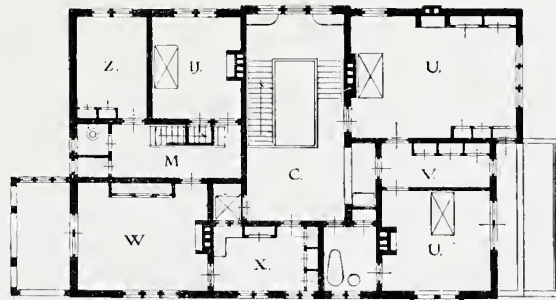
PLAN 1 ste VERDIEPING.
