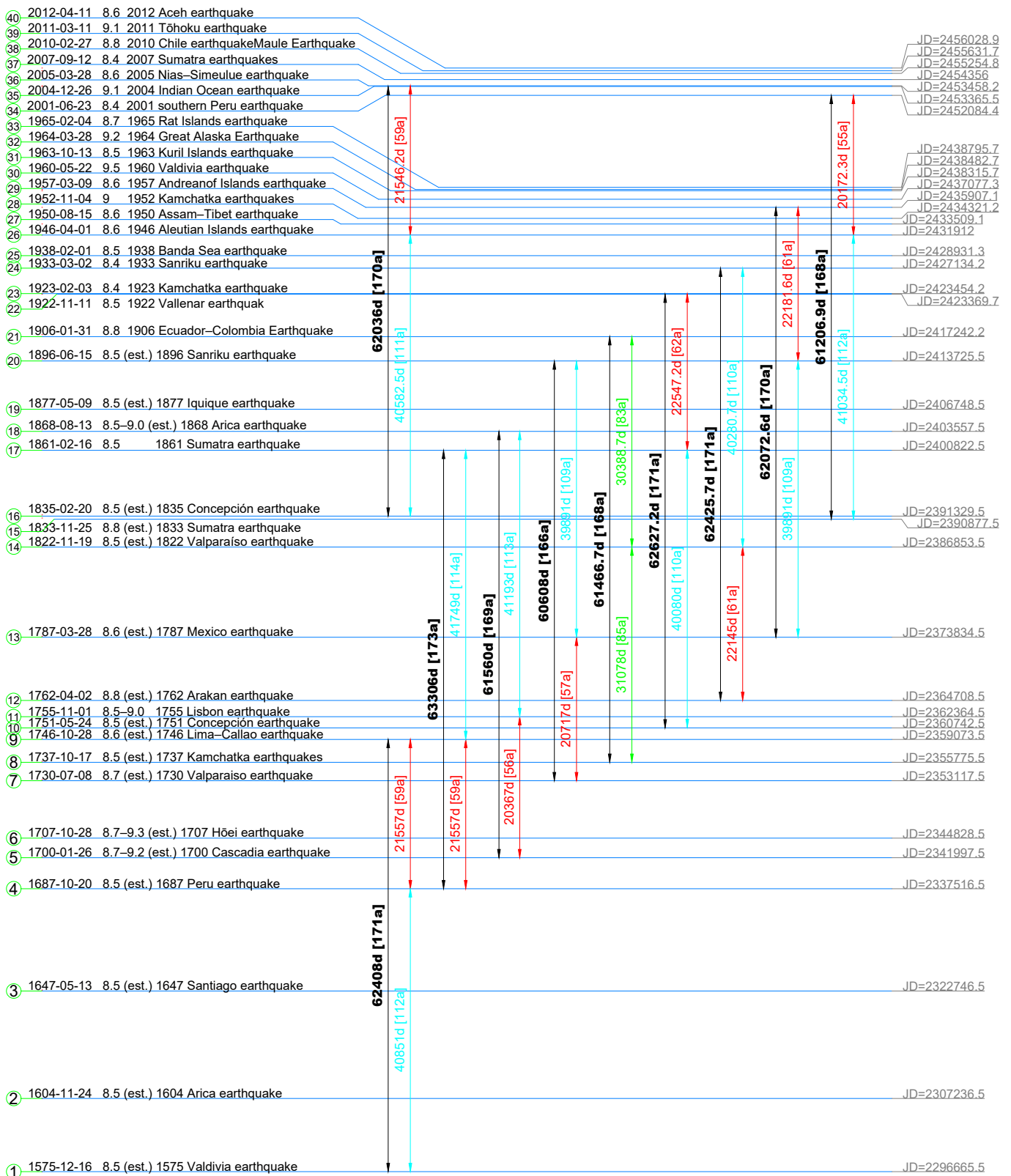
Fig.1.3 Relationship between the 167, 171-year cycle and the 59-year cycle in 40 major earthquakes (M>8.4)
