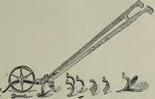
No. 16 Planet Jr. Single Wheel Hoe. Price, with attachments shown in cut, $5.85
