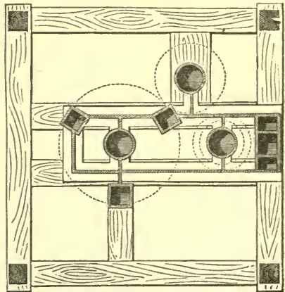
Plan of bed-plate; scale \frac{1}{4} in. to 1 foot.
