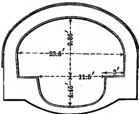
FIG. 5. OLD STYLE.
