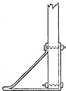
FIG. 8.—GRADE-ROD.
