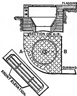
FIG. 6. IRON CURB INLET
