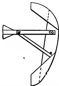
FIG. 9.—INSPECTOR'S TEMPLET FOR EGG- SHAPED SEWER.
