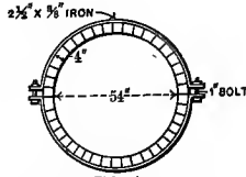
FIG. 4. WOODEN OUTLET SEWER NEW YORK CITY.
