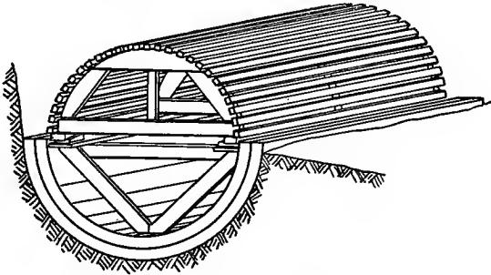
FIG. 25.—CENTRE FOR BRICK SEWERS.
