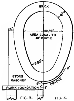
FIG. 3. IN SOFT EARTH FIG. 4. IN FIRM EARTH BRICK SEWER
