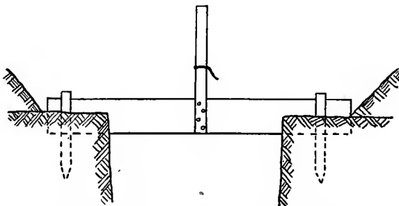
FIG. 5.—METHOD OF SETTING GRADE-PLANK.
