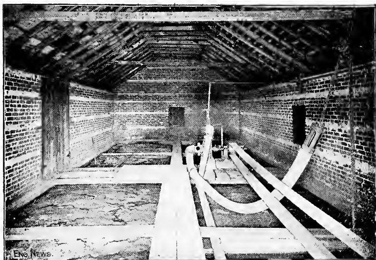
FIG. 38—INTERIOR OF CHAMPAIGN, ILL., SEPTIC TANK. (From Engineering News .)
