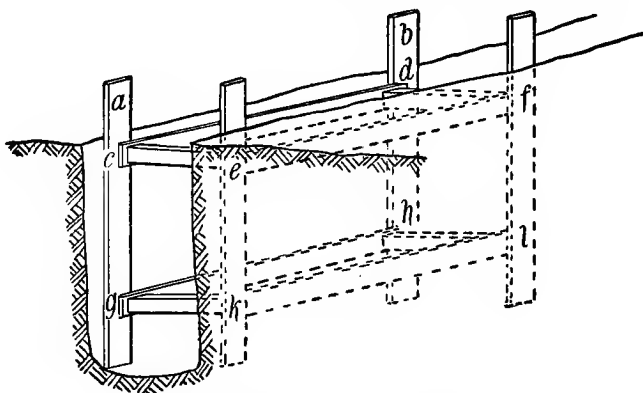
FIG. 13.—SKELETON SHEATHING.
