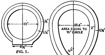
CEMENT PIPES
