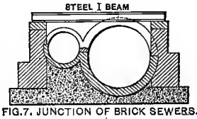
FIG. 7. JUNCTION OF BRICK SEWERS.
