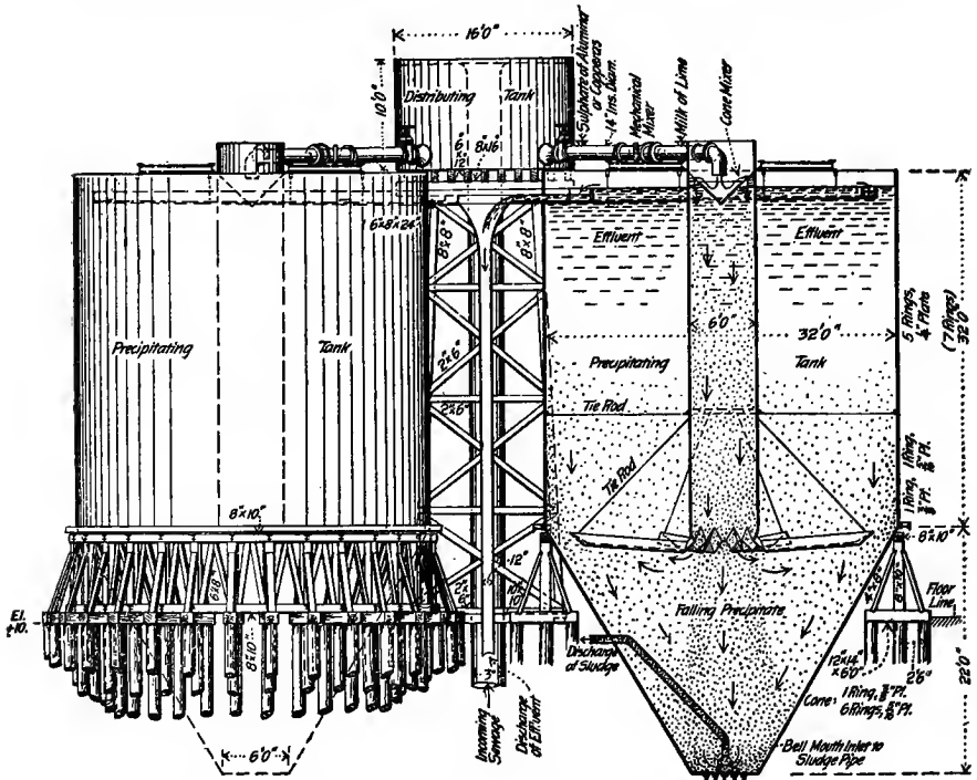
FIG. 37.—ELEVATION AND SECTION OF RECEIVING AND PRECIPITATING TANKS.
