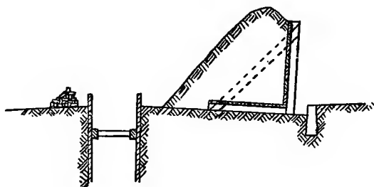
FIG. 11.—EXCAVATION-PLATFORM.
