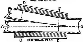
SECTIONAL PLAN E FIG. 6. JUNCTION OF 8 FT. AND 11 FT. SEWERS.
