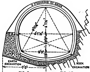
FIG. 9. WEST SIDE TRUNK SEWER, ROCHESTER.
