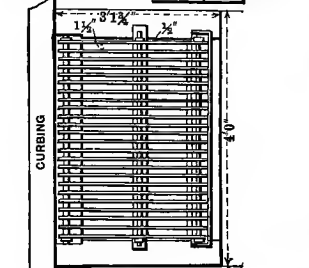
FIG. 4. WROUGHT IRON INLET GRATING.
