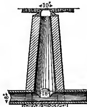
FIG. 11. BRICK LAMPHOLE.
