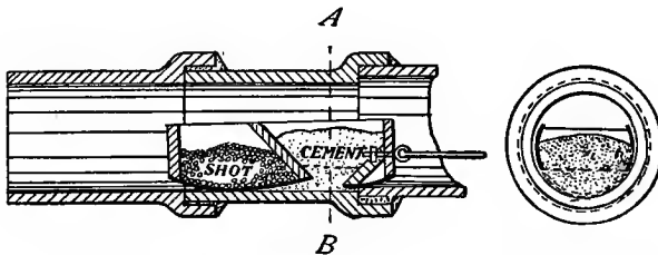
FIG. 10.—INVERT-FORMER.
