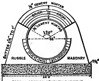
FIG. 8. SALT LAKE CITY. OUTLET SEWER.
