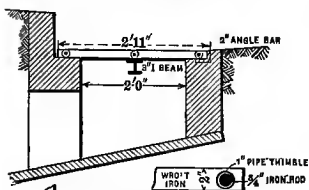
FIG. 1. FLUSHTANK
