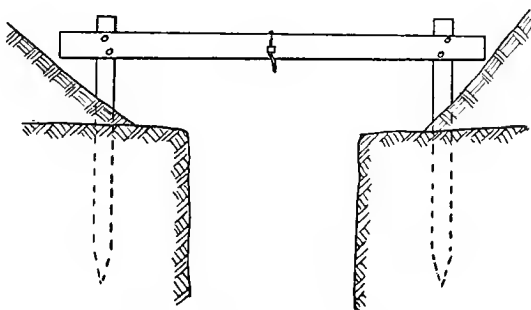
FIG. 6.—METHOD OF SETTING GRADE-PLANK.
