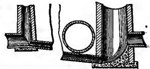
FIG. 6. INVERTED SIPHON.
