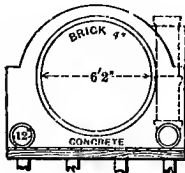
FIG. 6. INTERCEPTING SEWER AND SUB-DRAIN. BALTIMORE, MD.
