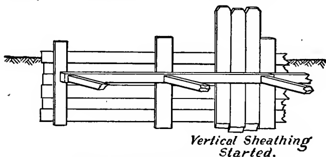
FIG. 16.—HORIZONTAL SHEATHING.
