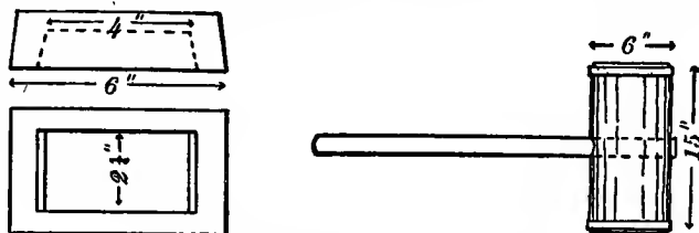
FIG. 15.—DRIVING-CAP AND MAUL.
