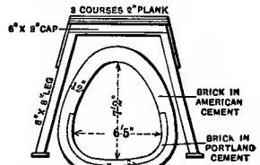
FIG. 7. IN TUNNEL METROPOLITAN SEWERS (BOSTON)
