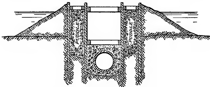
FIG. 31.—COFFER-DAM PUDDLE-WALLS.
