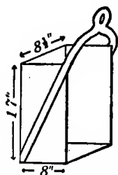
FIG. 23.—HOD FOR LOWERING BRICK.
