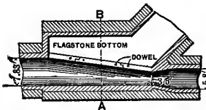
FIG. 3. STORM OVERFLOW, DENVER, COLO.
