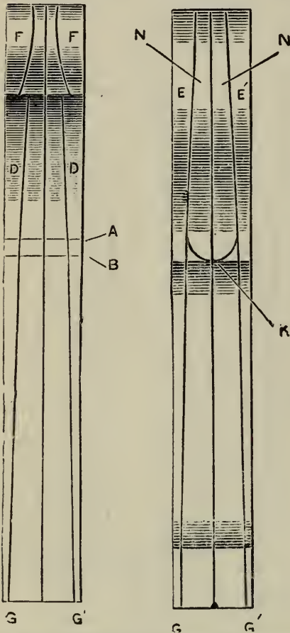
FIG. 163. — Neck Block marked for cutting out (back and front view).
