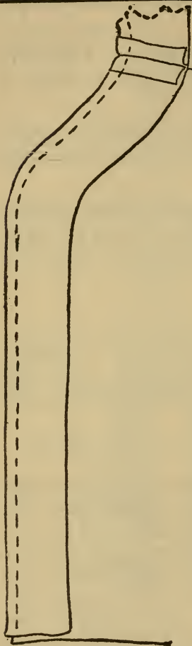
Fig. (38) The first stitching in facing the front of the pajamas
