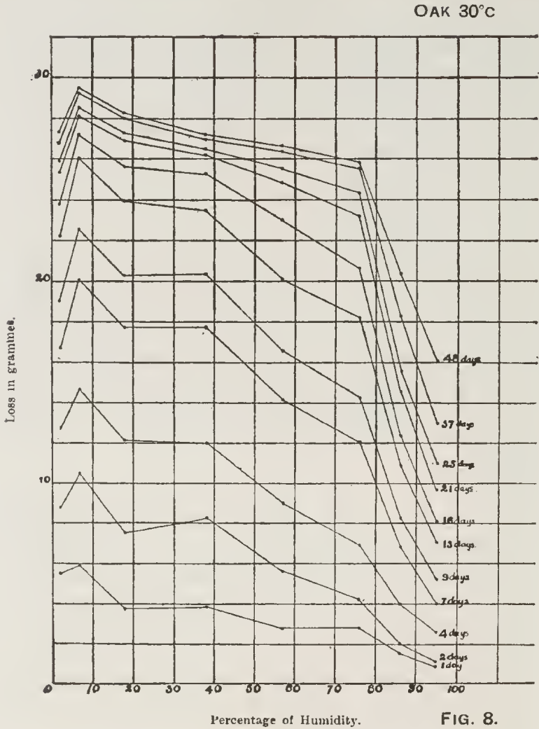
FIG. 8. TYPICAL SERIES OF LOSSES IN WEIGHT OF BLOCKS, DRYING AT VARIOUS HUMIDITIES.
