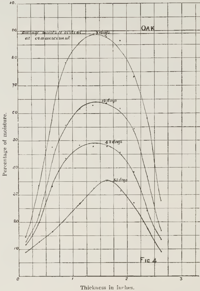
GRAPHS ILLUSTRATING THE PROGRESSIVE DRYING OF 3 IN. TIMBER AT 40°C AND 50% HUMIDITY.
