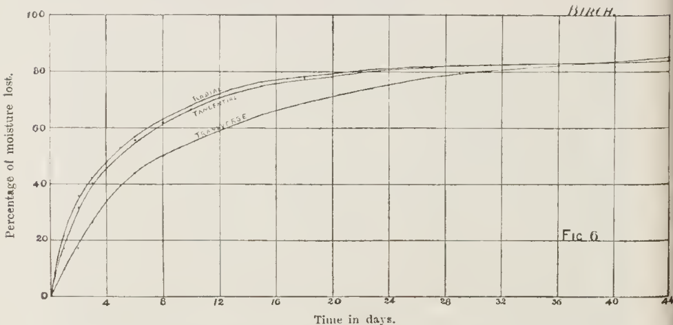
CURVES OF LOSS FOR BLOCKS OF BIRCH 1\frac{3}{8}'' \times 1'' \times 5''
