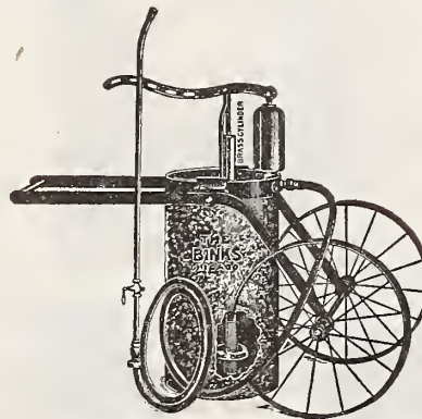
The Binks No. 21 Whitewash and Spray Machine
