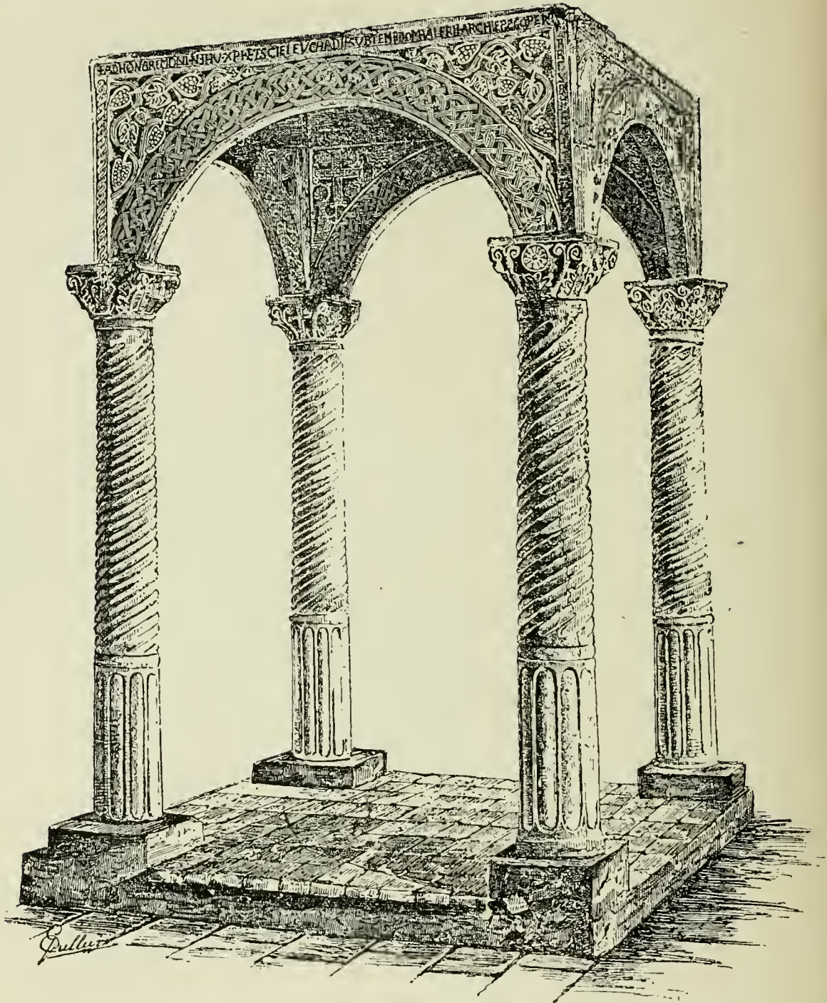
FIG. 104.—Ciborium of S. Elucadius in S. Apollinaris, near Ravenna—A.D. 806-816.
