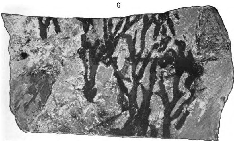
NIAGARAN GRAPTOLITES.
