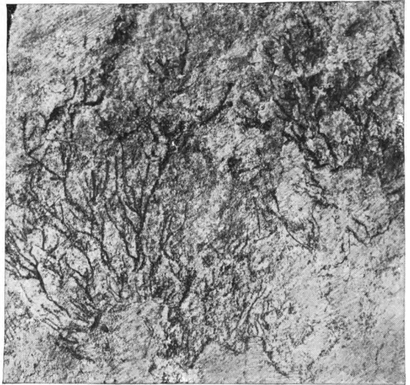
NIAGARAN GRAPTOLITES.
