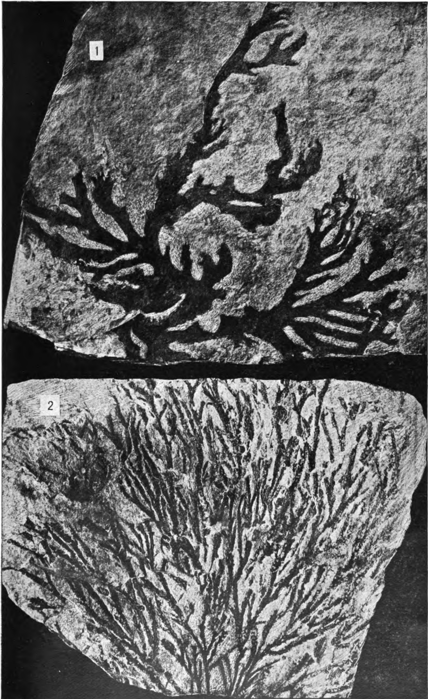
NIAGARAN GRAPTOLITES.
