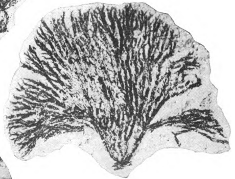
NIAGARAN GRAPTOLITES.
