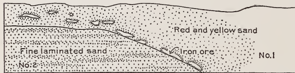
FIGURE 6.—Diagrammatic section of strata near Atlanta, Cass County.
