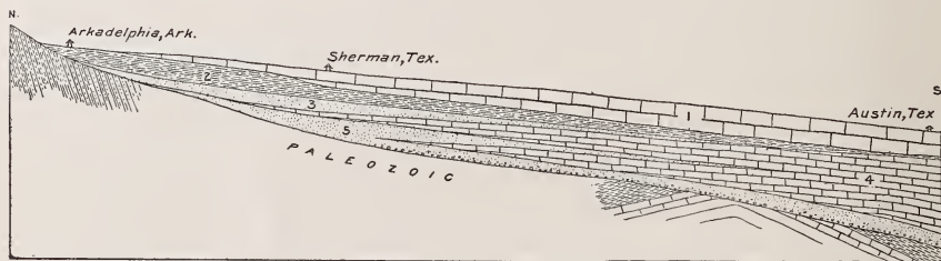
FIGURE 1.—Diagrammatic section of the Cretaceous rocks in northern Texas and southwestern Arkansas. (After Taff.) 1, White chalk; 2, blue marl; 3, sands at base of Upper Cretaceous; 4, Lower Cretaceous limestone; 5, sand at base of Lower Cretaceous. Reproduced from Twenty-second Ann. Rept. U. S. Geol. Survey, pt. 3, 1902, p. 697.
