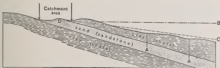
FIGURE 3.—Diagram showing the common arrangement of factors producing artesian wells. A, artesian wells; B, head of water if there were no loss by resistance or leakage; C, actual head of hydraulic gradient; D, ground-water table at outcrop.
