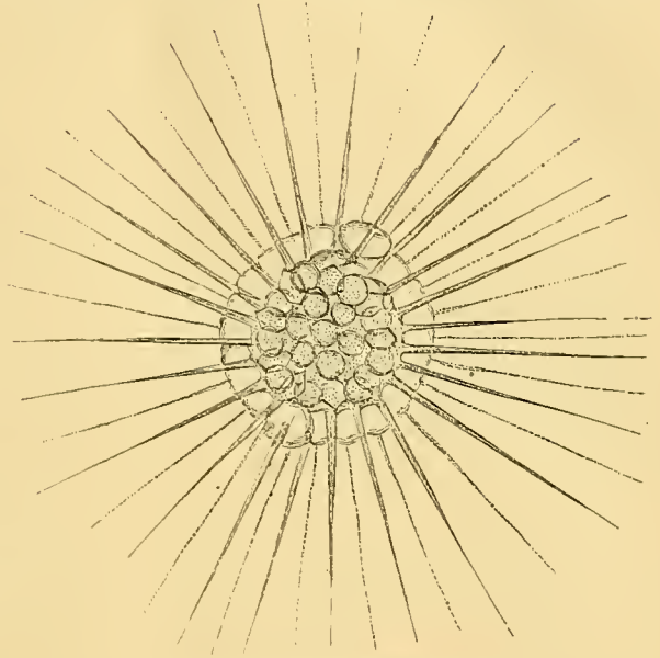
Fig. 13.— Actinospherium Eichhornii .
