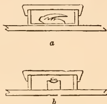
Fig. 37. Pill-box cells.
