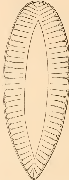
Fig. 132. Surirella elegans × 400.
