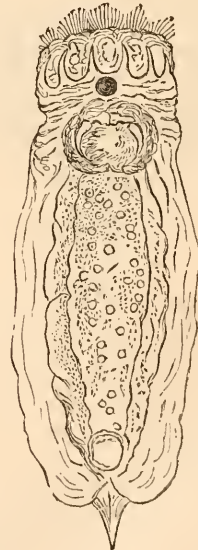
Fig. 118. Anuraea heptodon × 380.
