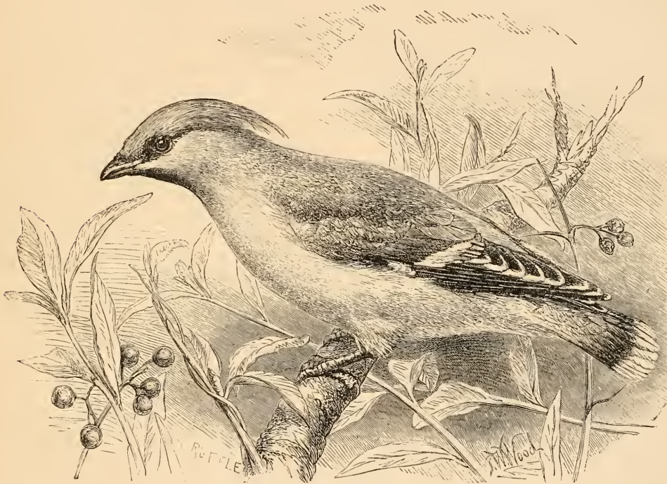
Fig. 196. THE WAXWING.
