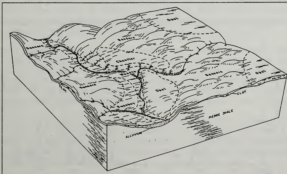
Figure 1. Patterns of soils in the Sansarc-Opal association.
