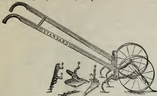
Standard No. 4 Double Wheel Hoe.
