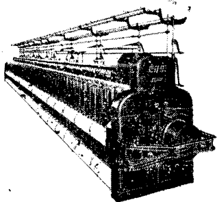
High Draft Inter. Frame
