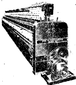
Wet Ring Doubling Frame
