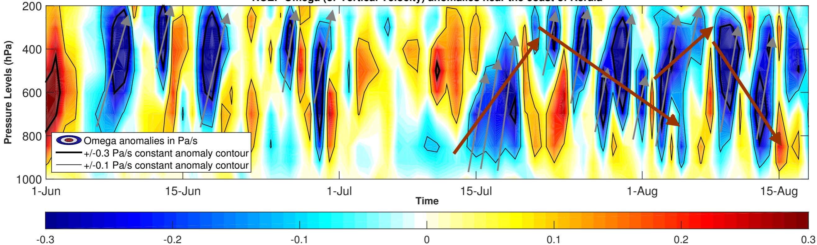
NCEP Omega (or Vertical Velocity) anomalies near the coast of Kerala
