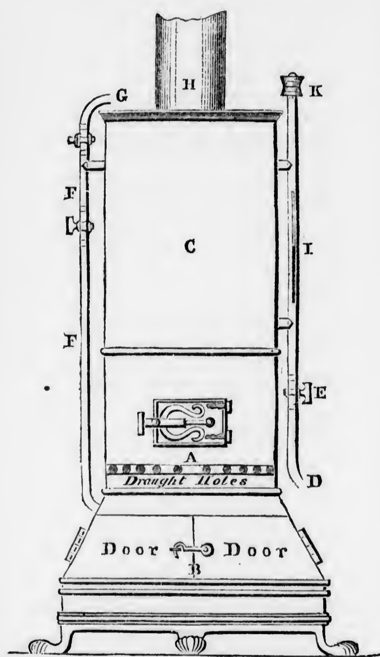
ELEVATION.—Scale 3/4-inch to 1 foot.
