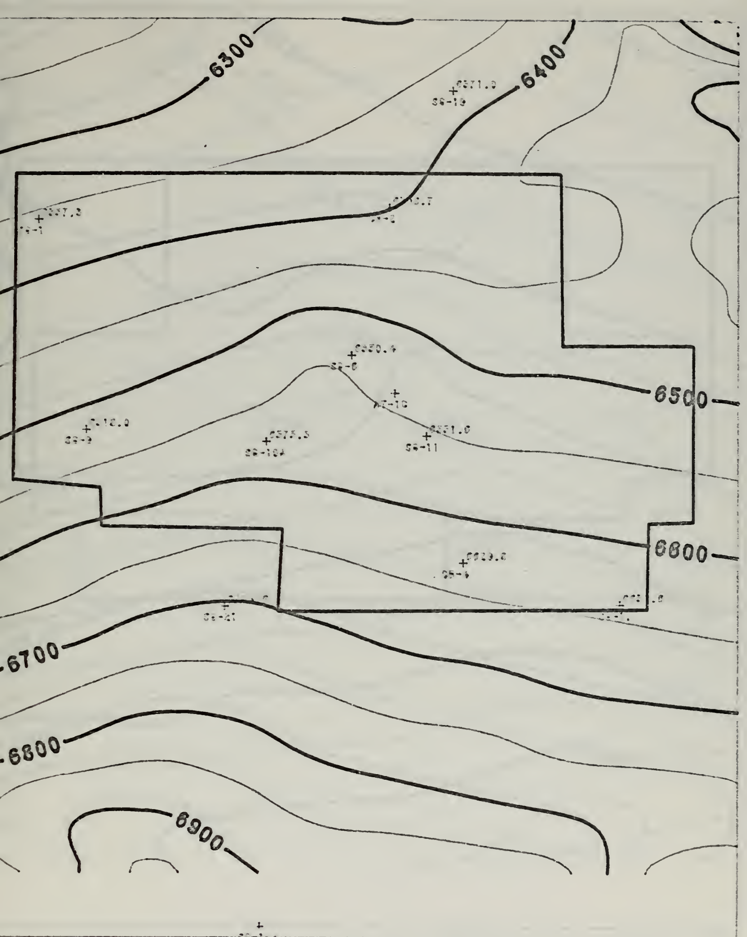
FIGURE A5.3.2B-10 Potentiometric Surface Map - Upper Aquifer, December 1977
