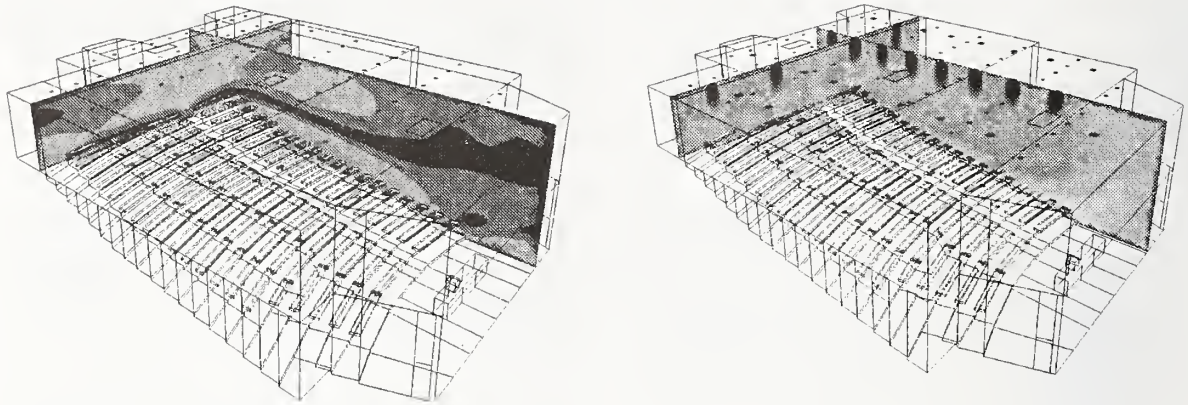
Figure 1. CFX provided CFD cross-sectional profiles of air velocity, which scales from 0.02m/s (blue) to 0.20m/s (red), in the displaced cooling scenario (Left) as well as the mixed cooling scenario (Right).
