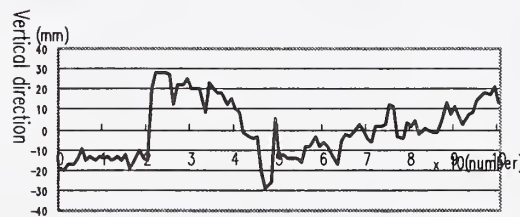
Figure 8: Values estimated by the system and measured values by Hydraulic differential
