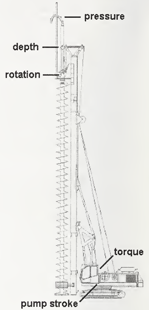
Figure 2 – CFA rig based sensors
