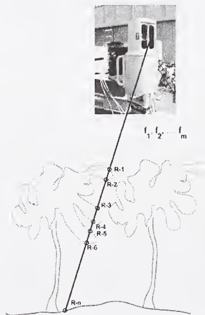
Figure 5: Due to beam divergence photons associated with a single “pixel” in a LADAR frame may represent significantly differing range data.
