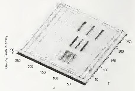
Figure 7. Reconstructed 25.4 mm (1 in) bars at 10 m.
