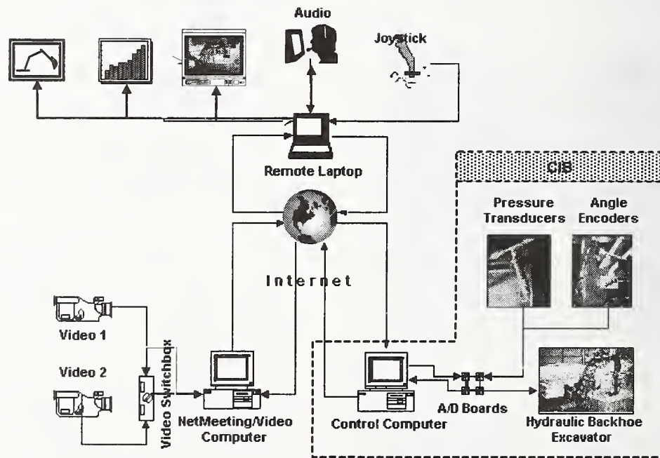
Fig 2. Schematic of Internet-Based-Operator-Training System
