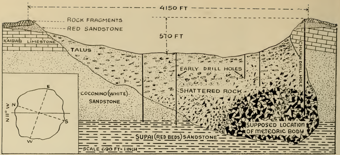
Cross-Section of Meteor Crater
