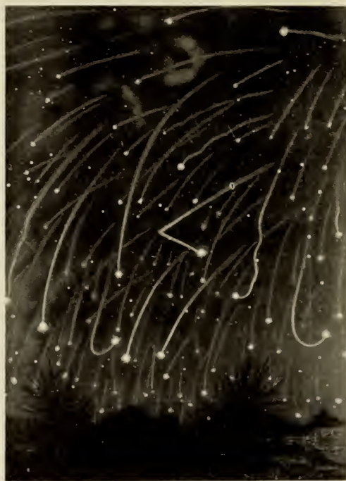
ARTIST'S CONCEPTION OF NOVEMBER METEORS NOVEMBER 13-14, 1866
