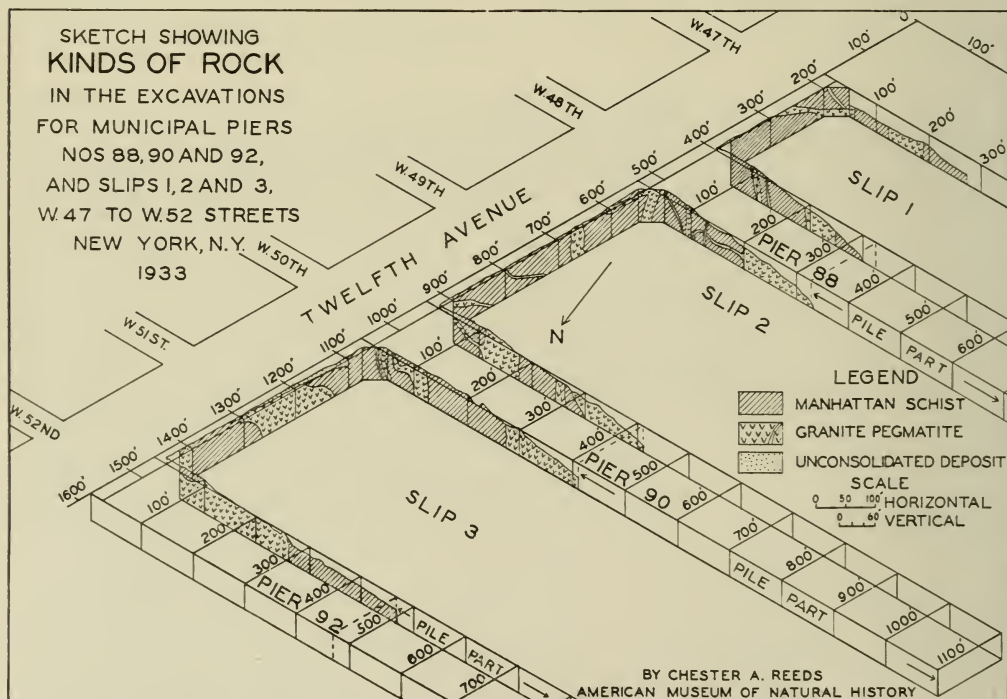
SKETCH SHOWING KINDS OF ROCKS IN 1100-FOOT PIERS, 88, 90 AND 92, NEW YORK. The metamorphosed Manhattan schist and the intruded granite pegmatites show a mixed relation. The unconsolidated deposits consisting of glacial deposits and river silt occur on the surface
