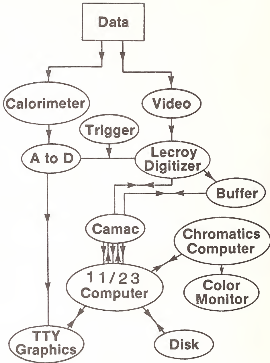
Figure 2. Block diagram of data collection system.
