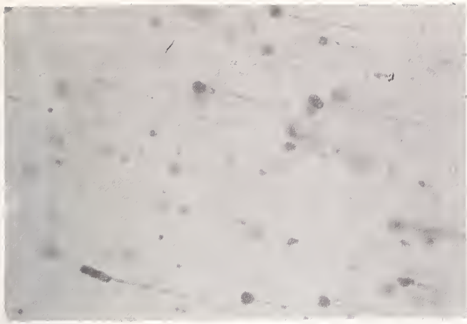
Figure 8. Bulk damage in LiF 3 shots, fluence 1.9\text{Jcm}^{-2} .
