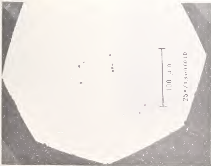
a. ZrO_2 ( \lambda/2 at 1.06\mu m ) on Fused Silica in 1 Torr N_2 (250x).
