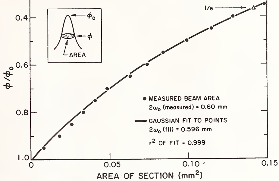
Figure 5. Spatial comparison of test beam to an ideal Gaussian. A good fit assures the validity of a comparison between theory and experiment.
