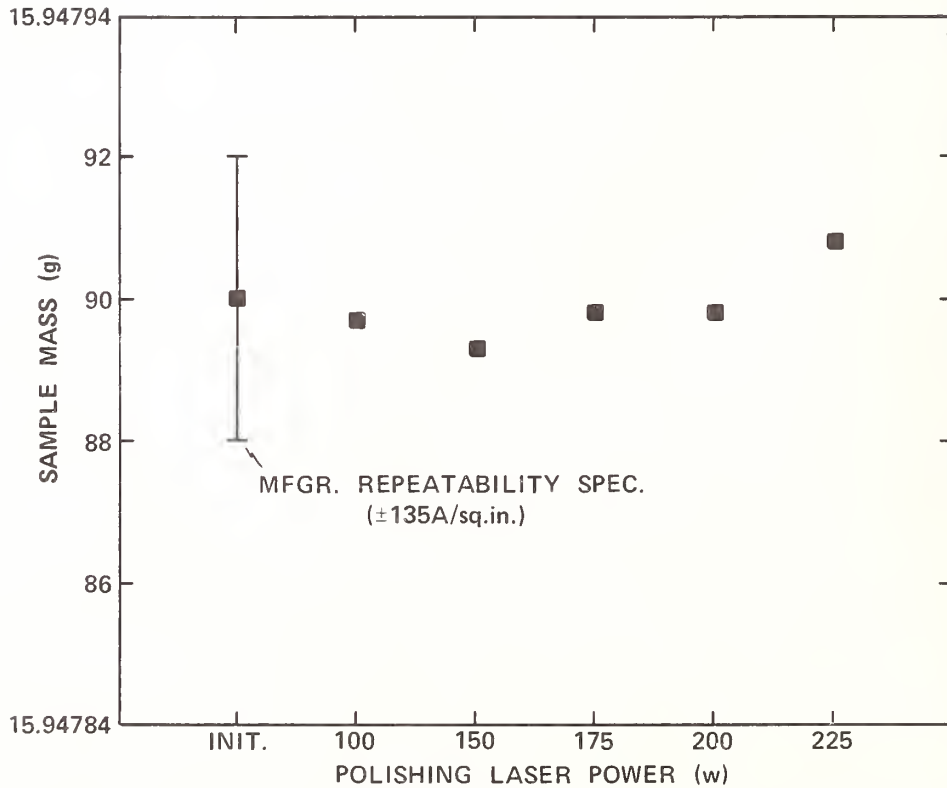
Figure 4. The mass of a sample of fused silica which was laser polished over a 1-inch-square area at successively higher laser intensities.
