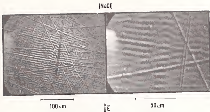
Figure 1. Laser Generated Ripple Patterns (LGRP) in NaCl. The above patterns were produced by normally incident 10.6 \mu\text{m} laser light on the exit surface of NaCl. The laser light was linearly polarized in the direction shown by \vec{E} . The higher power photo on the right illustrates that the ripples are associated with defects normal to \vec{E} whereas scratches parallel to \vec{E} have no ripples associated with them.
