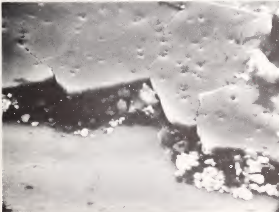
Figure 13. Cracked TiC coating on SS304 after irradiation with 1096 MW/cm 2 . The bottom part shows removal of a surface layer. Along the edges of the removed TiC area, cracking follows a narrow band of arc craters.
