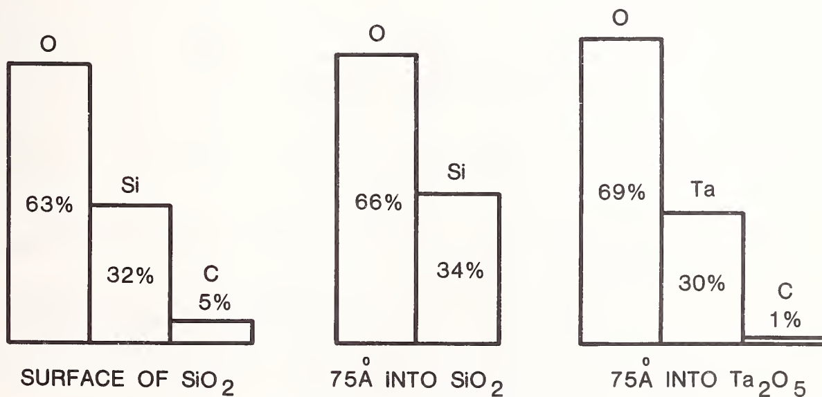
Figure 4. Composition of nominal SiO_2 and Ta_2O_5 films.
