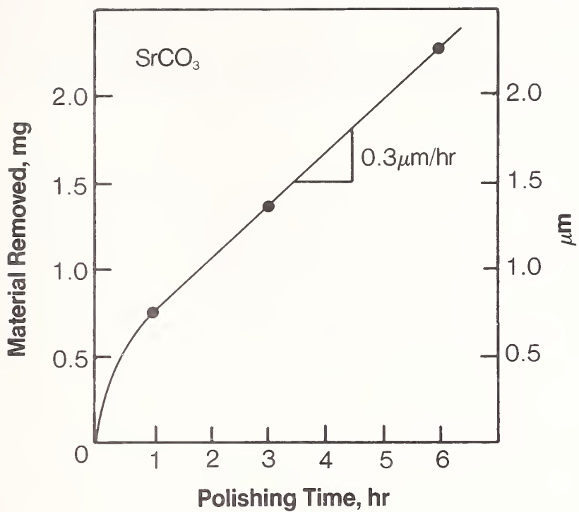
Figure 2. Weight loss of fused silica during dry mechanochemical polishing with SrCO 3 .
