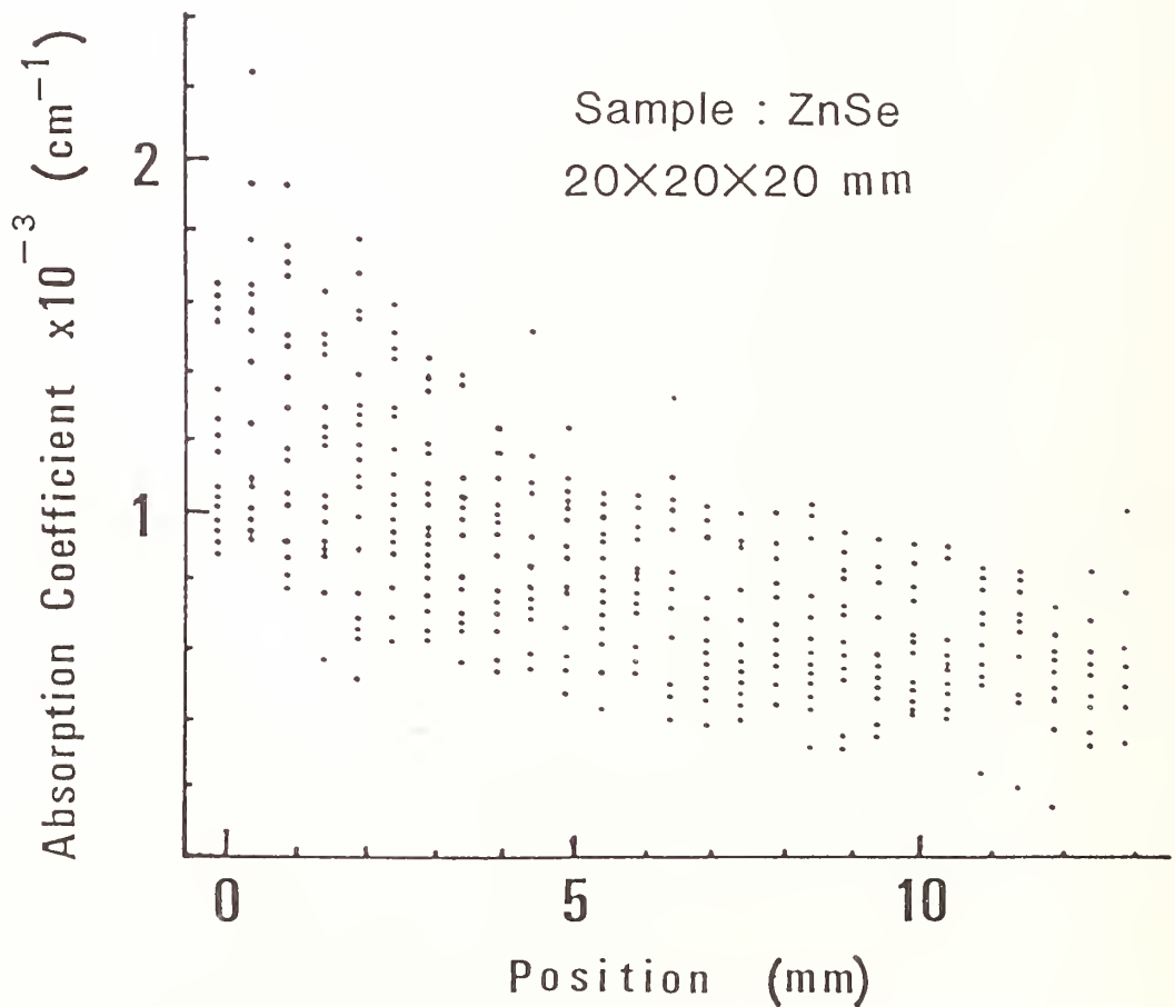
Figure 8. Distribution of the bulk absorption.
