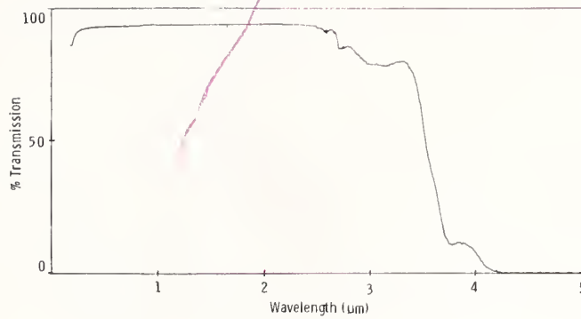
Figure 1. Spectral transmission of Suprasil W-1. Sample thickness is 13 mm.
