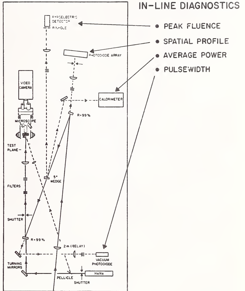
Figure 1. Line drawing of the Los Alamos laser damage test facility.
