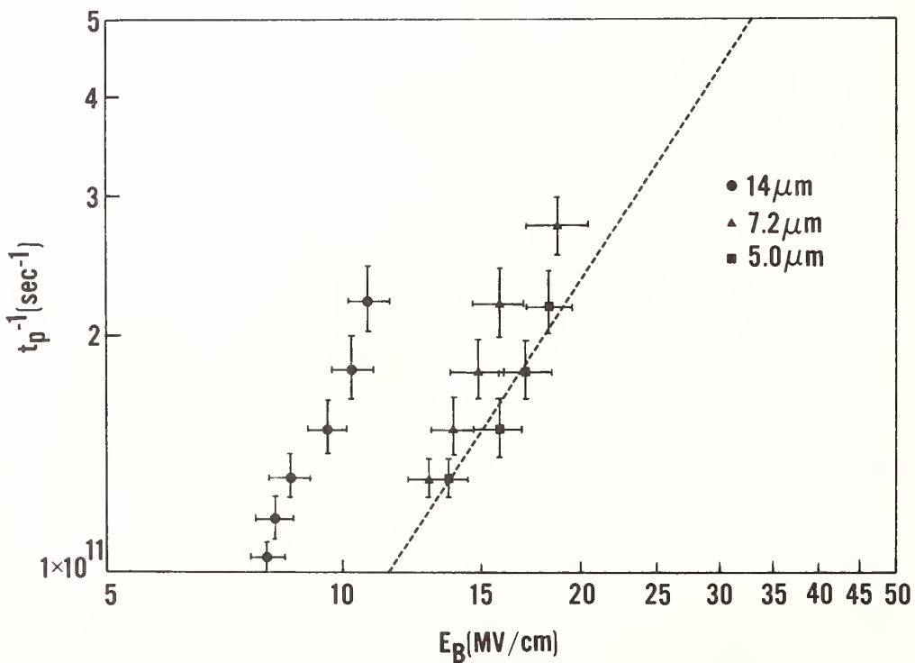
Figure 4. Pulsedwidth dependence of E_B in \text{NaCl} at 1.05 \mu\text{m} . The slope of the least square linear fit to each of the three sets of points is approximately 0.5. This indicates an inverse square root of pulsedwidth dependence of E_B for this pulsedwidth range ( t_p < 10 psec).
