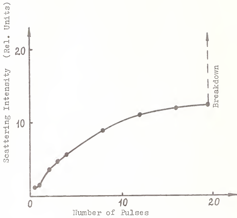
Figure 2. Scattering intensity of ruby-laser radiation versus the number of pulses at the multiple-shot damage in PMMA at the incident intensity. I = 0.5I_1 .
