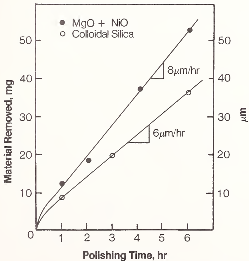
Figure 3. Weight loss of fused silica during mechanochemical polishing with slurries of colloidal silica and NiO and MgO.
