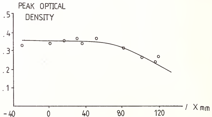
Figure 3. Peak optical density of Dylux film plotted against distance beyond the lens.
