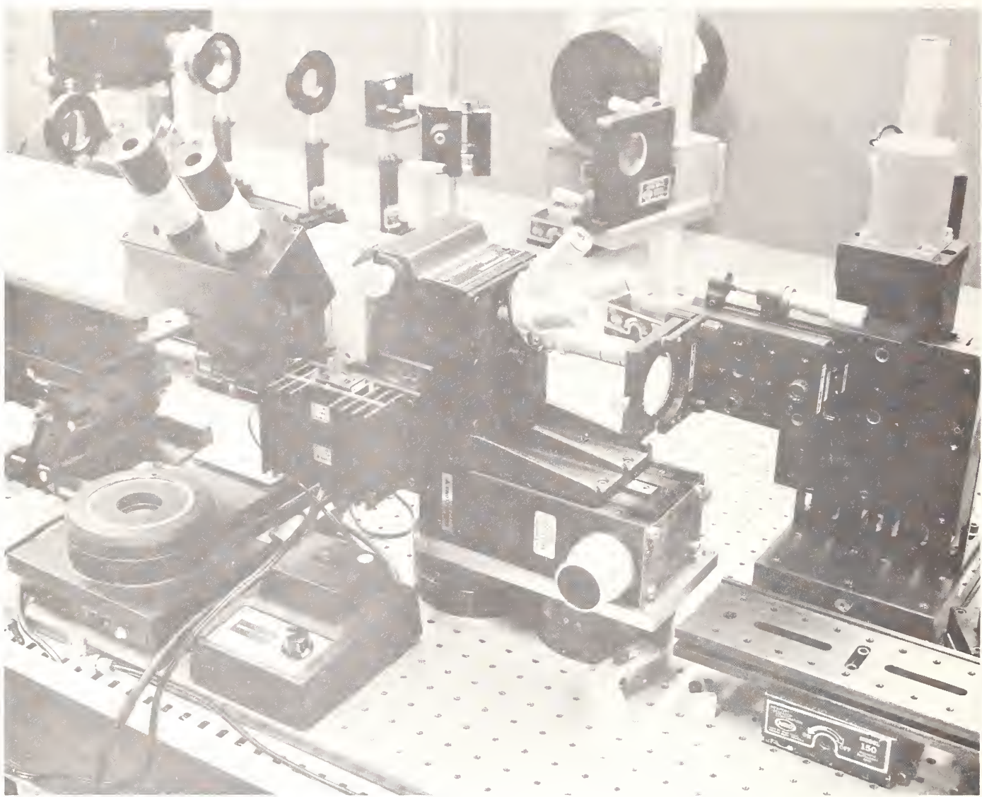
Figure 2. Photograph of test section. Sample holder on X-Y steppers is located a few cm from objective of microscope (center). Beam enters from right.
