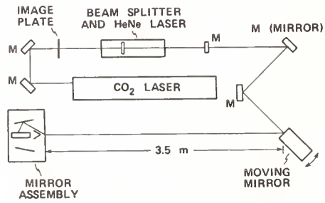
Figure 8. Diagram of the CO 2 laser polishing apparatus.
