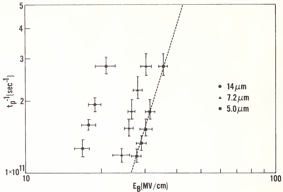
Figure 3. Pulsedwidth dependence of E_B for \text{SiO}_2 at 1.05 \mu\text{m} . The three sets of points correspond to different focal spot radii and the relatively large displacement of the three sets of points is indicative of a large spot size dependence in the damage threshold. The slope of the least square fit for each set of points is approximately 0.3 for this pulsedwidth range ( t_p < 10 psec).
