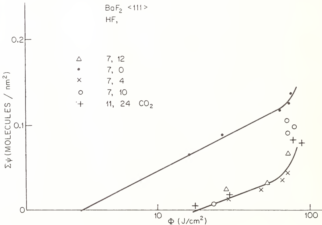
Fig. 6 Cumulative LID fluence of mass 18 (H 2 O) as a function of axial energy density for an N/1 experiment on (111) BaF 2 . D_{1/e^2} = 380 \mu\text{m} at HF and CO 2 . Irradiated sites are designated by their coordinates in mm.
