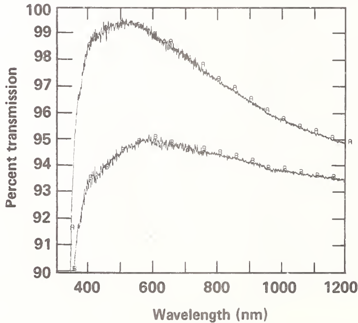
Figure 7. Two surface transmission of 1-cm thick primary green part contaminated with doctylphthalate during 2 months storage (B) and after ethyl alcohol rinse (A).
