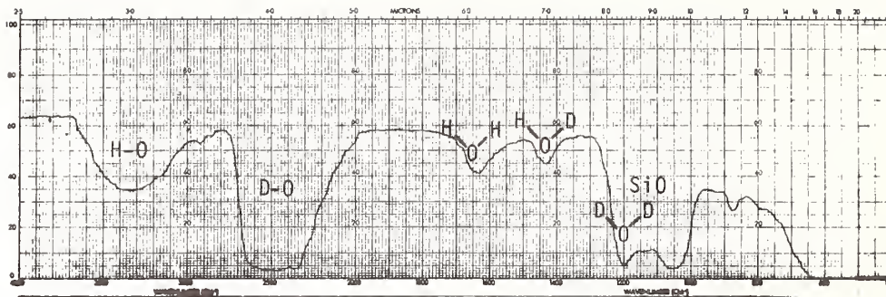
Figure 10. Sample #2 Internal reflection 100Å SiO 2 , 5000Å ThF 4 on ZnSe \theta=45^\circ 25 reflections Heated >90^\circ\text{C} 2 hrs. in D 2 O vapor
