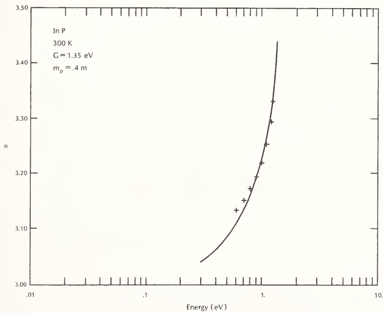
Figure 2. Theoretical results for InP for a sample with carrier concentration n_a = 5 \times 10^{16} \text{ cm}^{-3} (solid line) plotted along with experimental results on a sample of the same carrier concentration obtained from Reference (7) (+++++).
