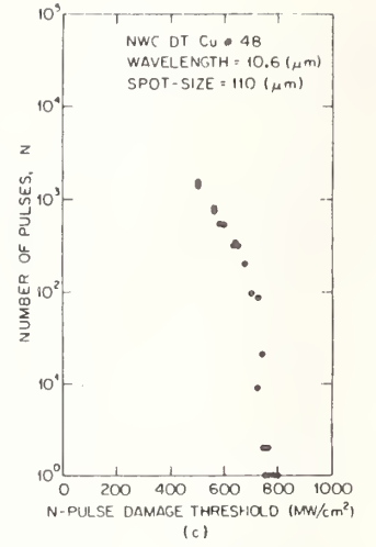
Figure 2. Measured \log N vs I_N for diamond-turned OFHC Cu irradiated at a) 0.532 \mu\text{m} b) 1.06 \mu\text{m} c) 10.6 \mu\text{m} .
