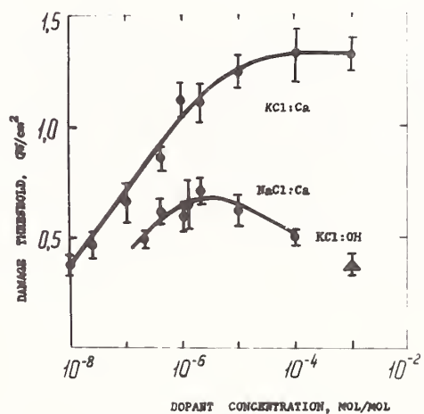
Fig. 2. Bulk damage threshold in NaCl and KCl samples versus Ca concentration. Triangle is the threshold for KCl-OH.
