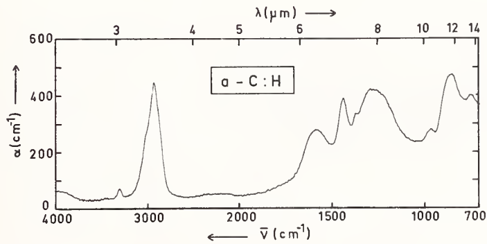
Figure 2: Infrared absorption coefficient of a-C:H.
