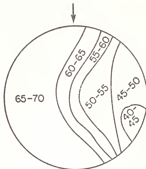
Figure 3. Transmission map of Vitreosil IR-1 sample #3949 showing approximate lines of constant transmittance. The sample was measured at 2.7 \mu\text{m} at various locations and showed the above extreme inhomogeneity.
