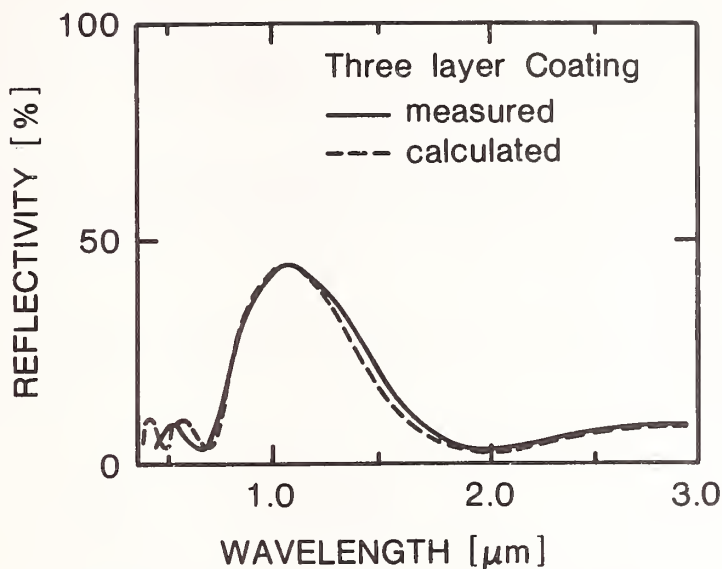
Figure 3. Comparison of calculated and measured reflectivities for quarter wave Ta_2O_5-SiO_2-Ta_2O_5 coating.
