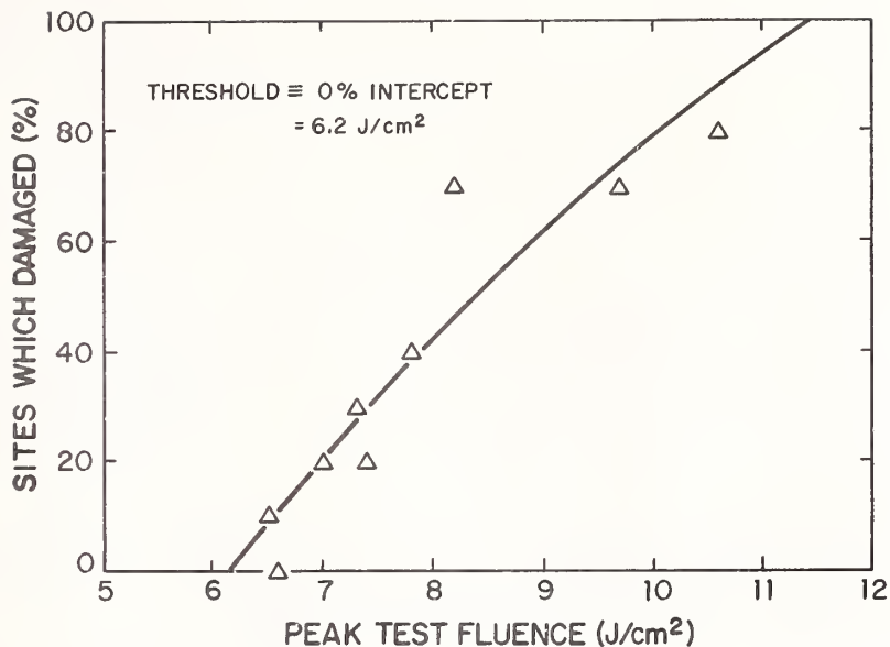
Figure 1. Results of a standard test at 308 nm of a Sc 2 O 3 /MgF 2 reflector. Each triangle represents the fraction of ten test sites which damaged at a particular test fluence. Damage threshold is the zero-probability intercept - 6.2 J/cm 2 .
