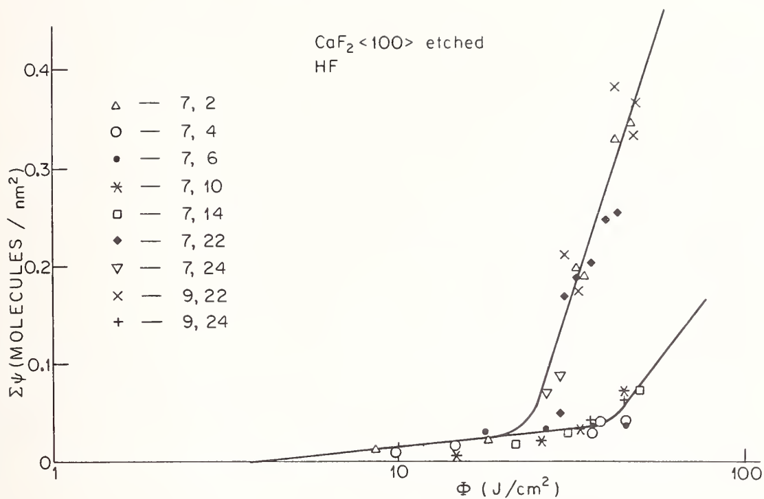
Fig. 3 Cumulative LID fluence of mass 18 ( H_2O ) as a function of axial energy density for a N/l experiment using the same system as Fig. 2. Each irradiated site is designated by its coordinates in mm.
