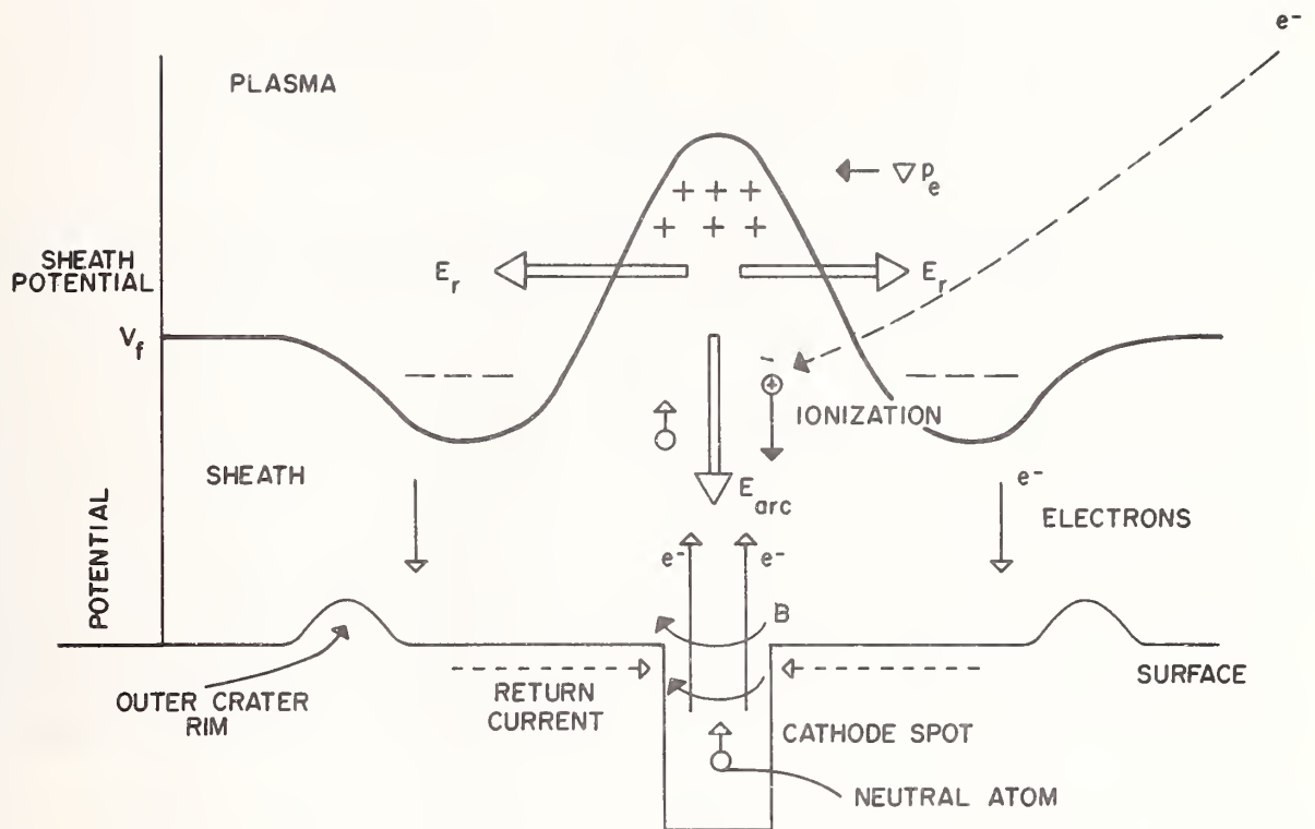
Figure 2. Unipolar arc model
