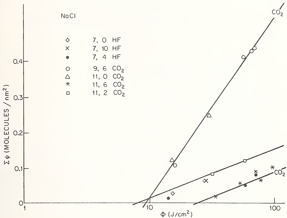
Fig. 7 Cumulative LID fluence of mass 18 ( H_2O ) as a function of axial energy density for an N/1 experiment on (100) NaCl. D_{1/e^2} = 380 \mu m at HF and CO_2 . Irradiated sites are designated by their coordinates in mm. (Back surface damage at the CO_2 wavelength is indicated by the CO_2 notation on two graphs.)
