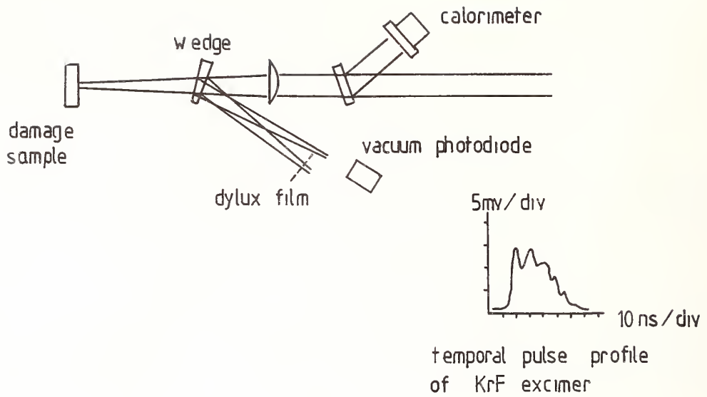
Figure 1. Experimental Arrangement.
