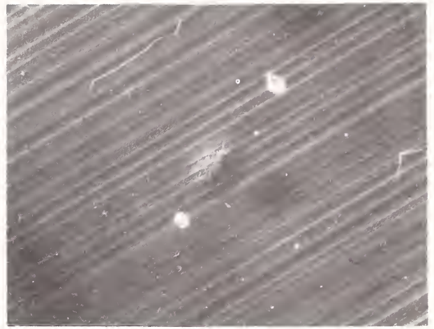
Figure 2. Nomarski micrographs of damage sites showing slip on a diamond-machined OFHC copper surface with the initial sample temperature at 133°K in (a) and 300°K in (b). No differences in morphology are evident.
