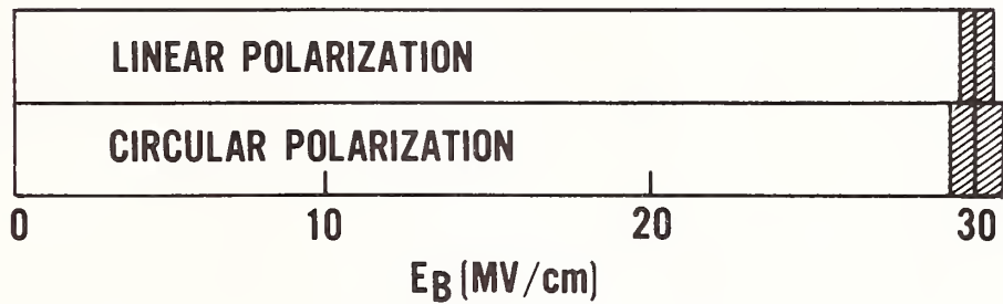
Figure 1. Polarization dependence of E_B for \text{SiO}_2 . The horizontal axis is E_B , the r.m.s. breakdown field corresponding to the peak on-axis irradiance at damage. P_B is the breakdown threshold power. Note the lack of polarization dependence for both wavelengths. The cross-hatched portions shown above are the relative uncertainties of the thresholds using the procedures given in Ref. 16.
