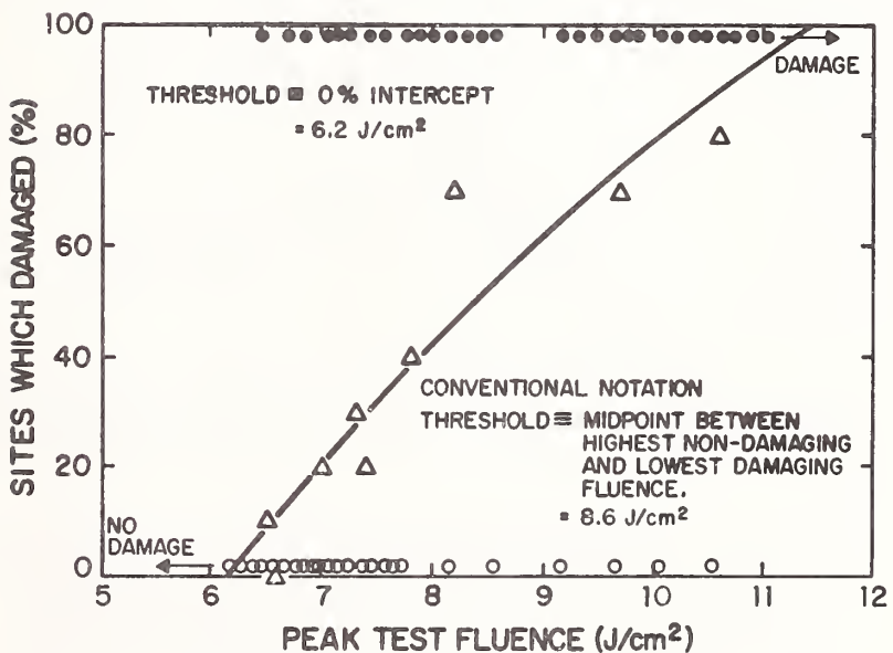
Figure 2. The data of figure 1 are replotted in the conventional manner (open and closed circles). As defined conventionally, threshold is 8.6 J/cm 2 .
