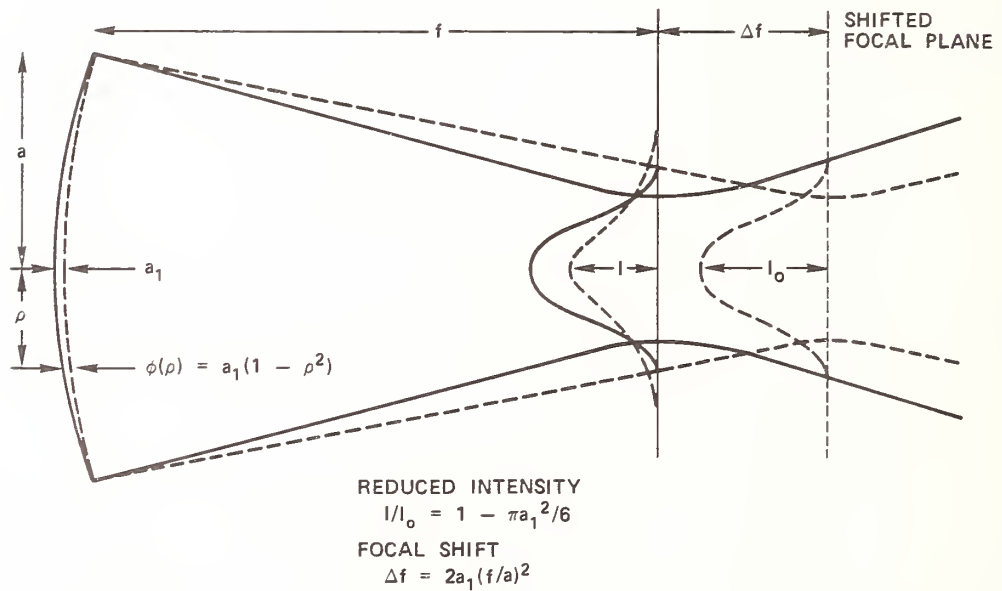
Figure 3. Drop in on-axis intensity I caused by spherical wave front error restored to I_0 by shifting focal plane to right.
