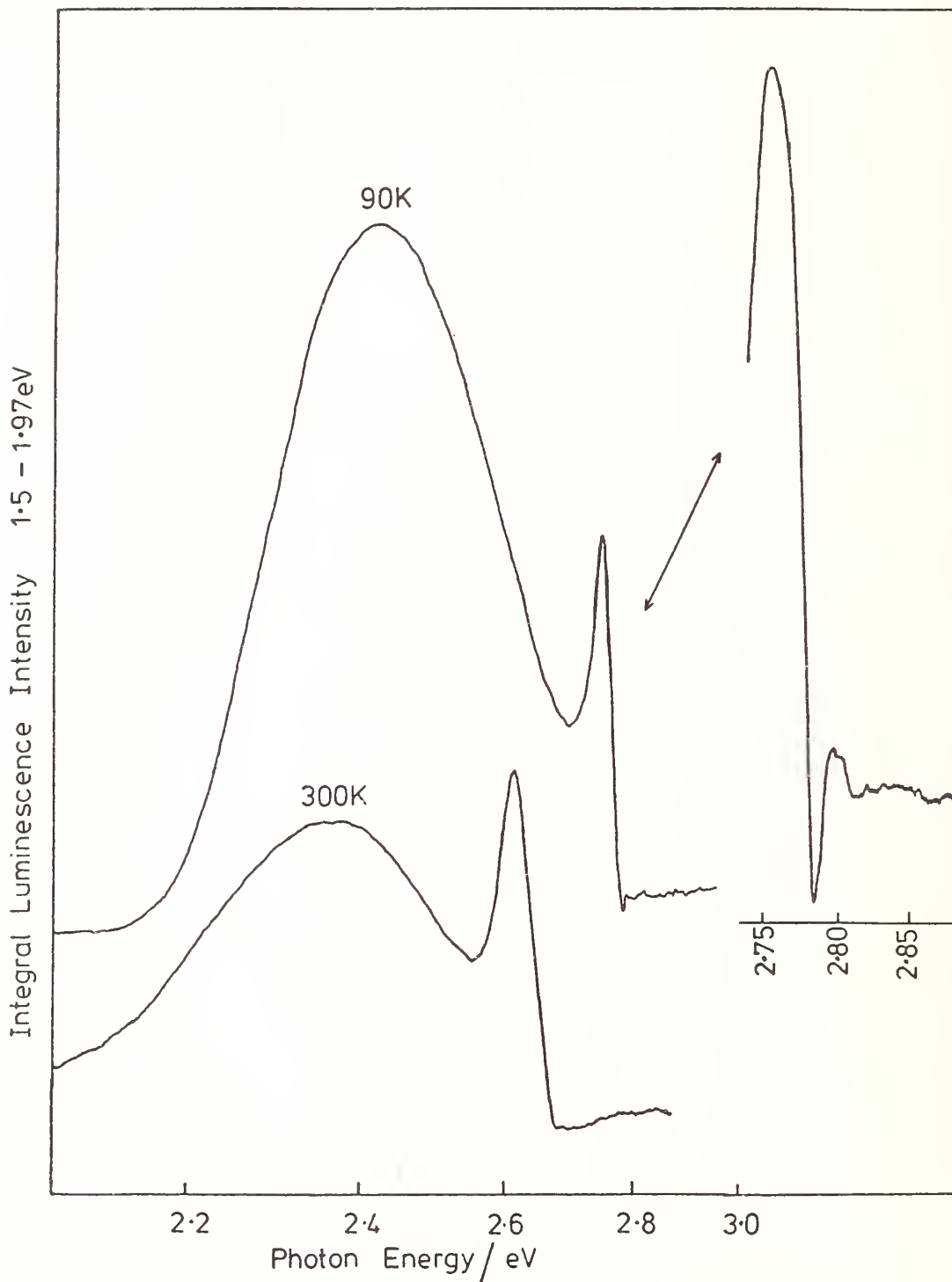
Fig 5. Photoluminescence Excitation Spectrum for Red Emission Process.
