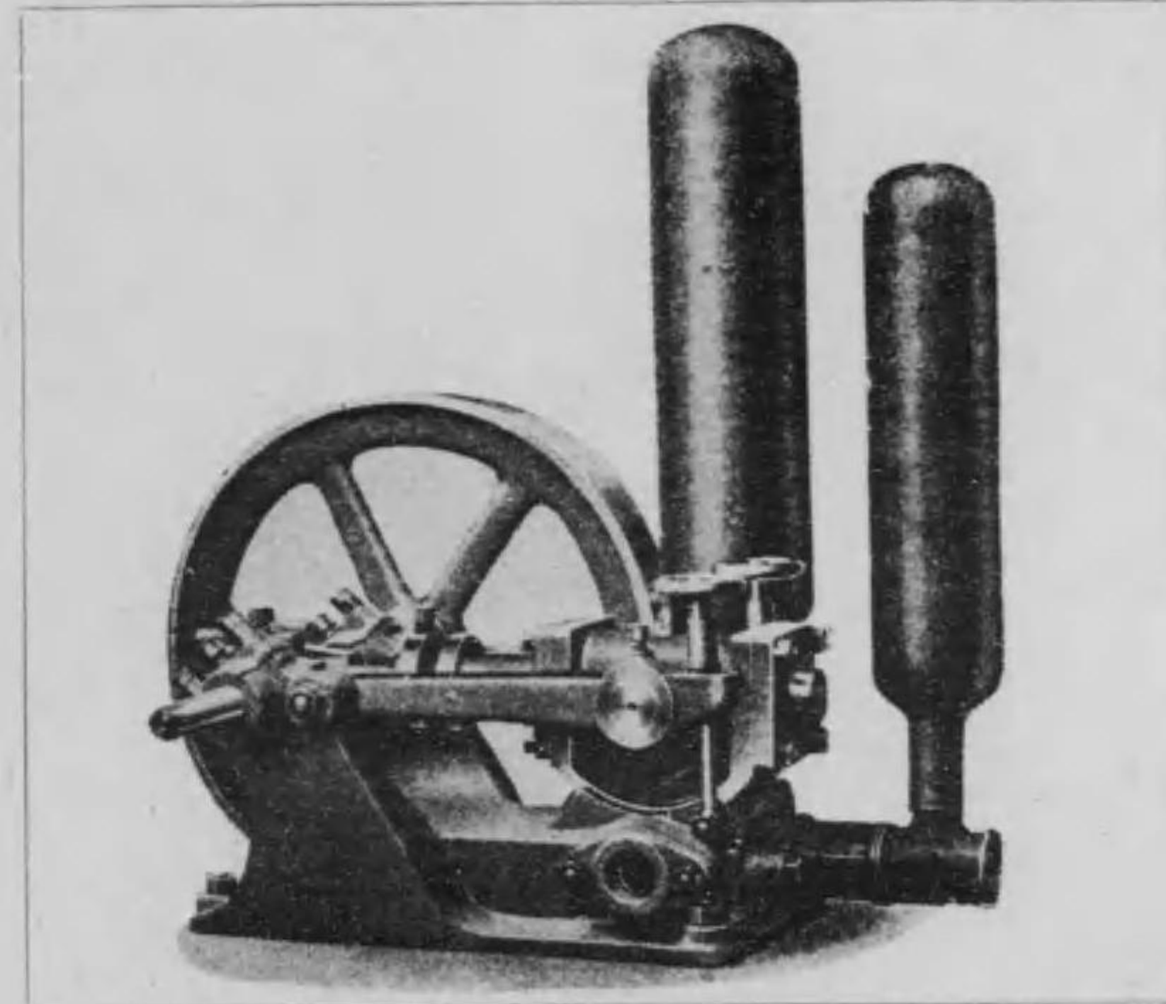
OSCILLATING DOUBLE-ACTING PISTON-PUMP (Without Valves) For Thickliquids.
