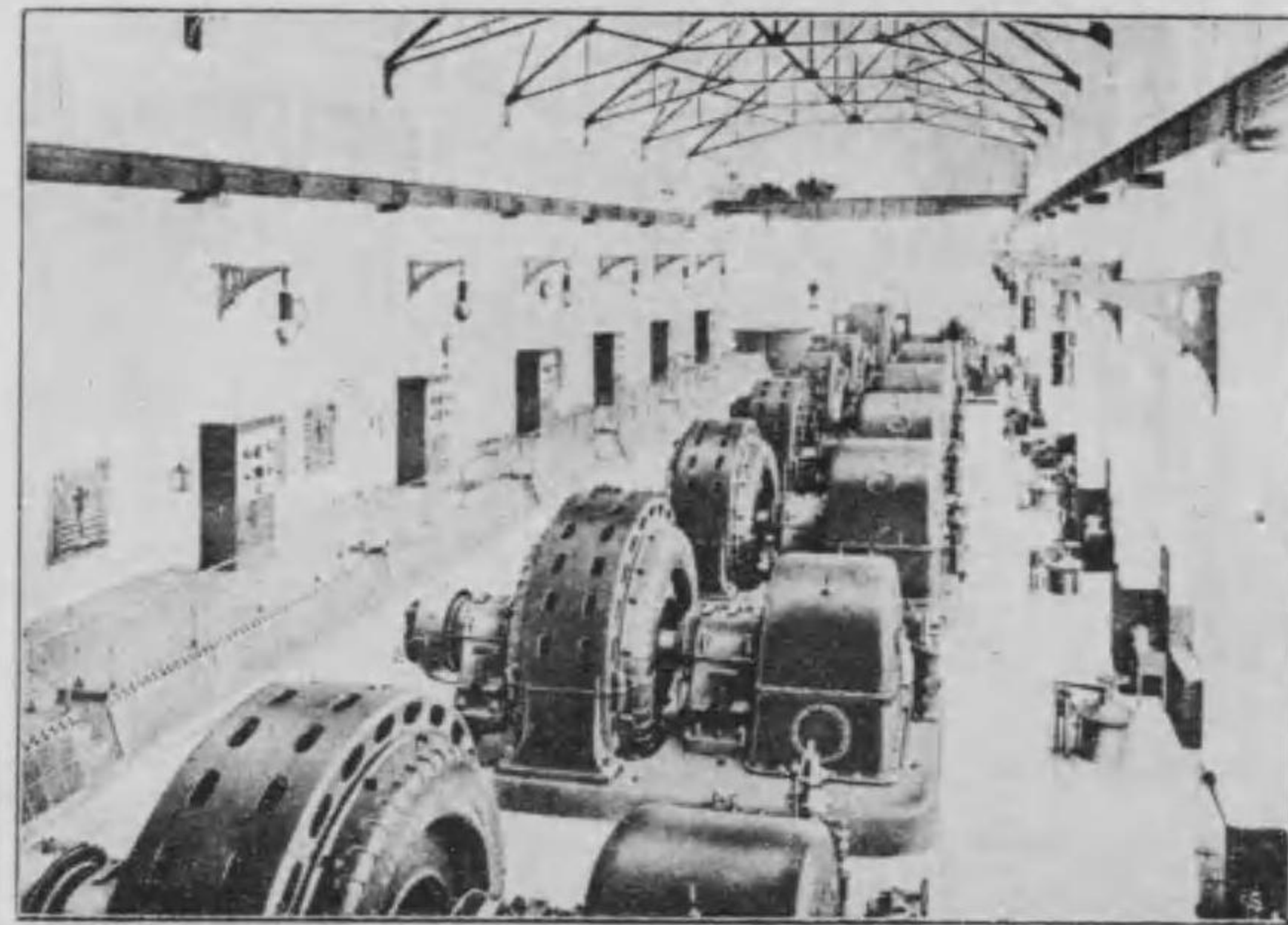
6 PELTON TURBINES of 7000 HP. each 2 PELTON TURBINES of 16000 HP. each HEAD 340 m., SINGLE WHEELS.
