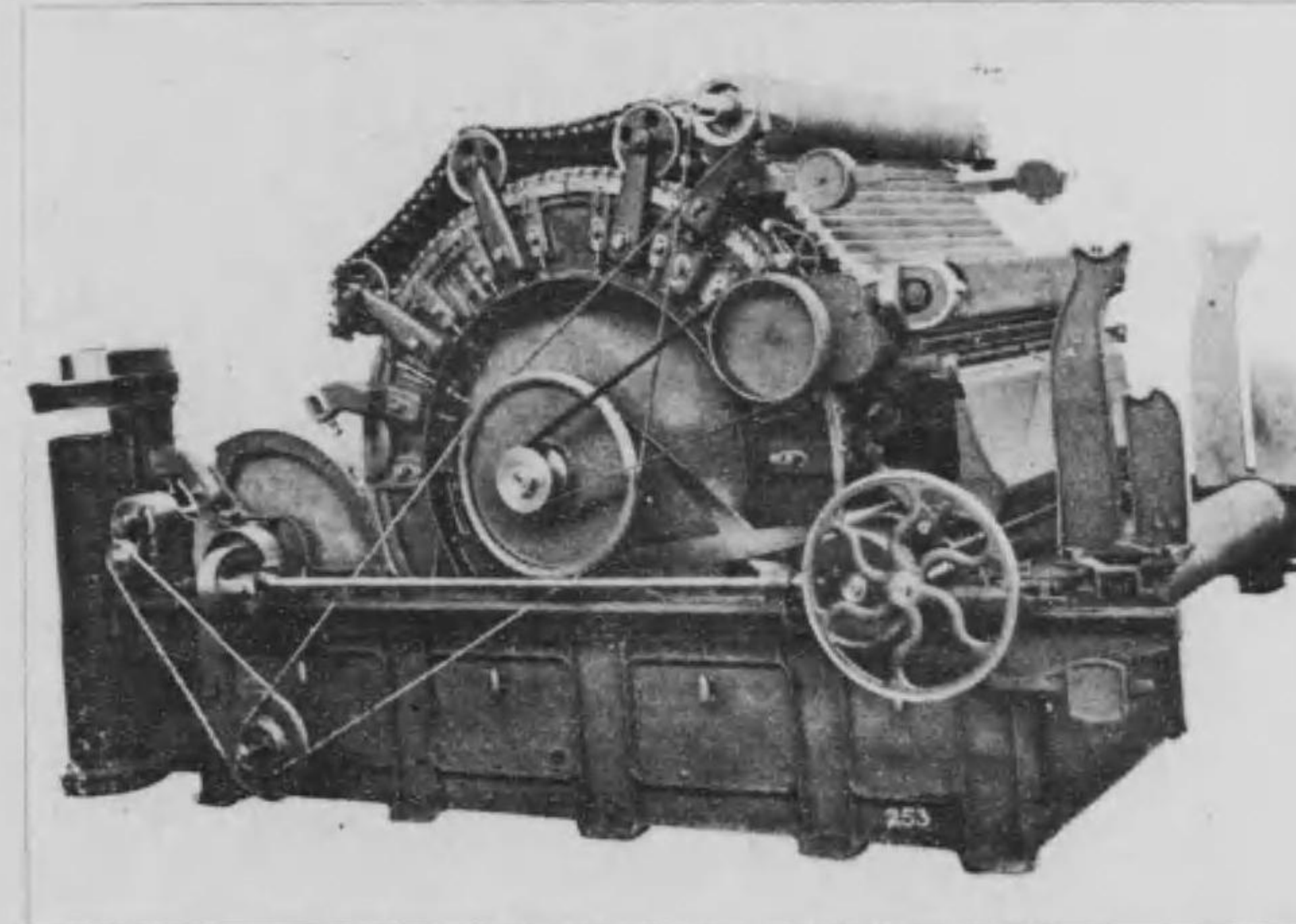
Carding Engine with 100 Revolving Flats.
