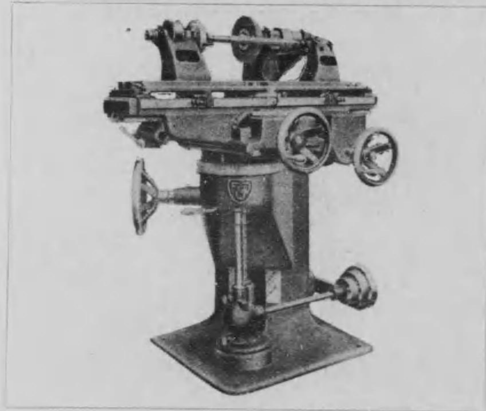
UNIVERSAL TOOL GRINDER "RAPID III"
