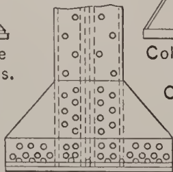
Built up Column Base for heavy loads.
