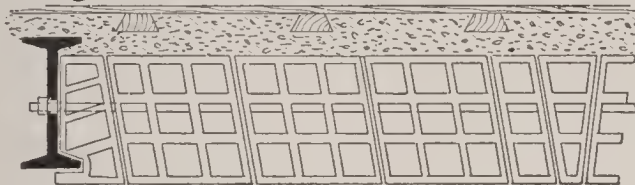
Fig. 3. Parallel Web or Side Construction.
