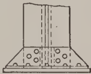
Column Base for light loads.
