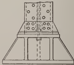
Column Base with Cast Iron or Cast Steel Base.
