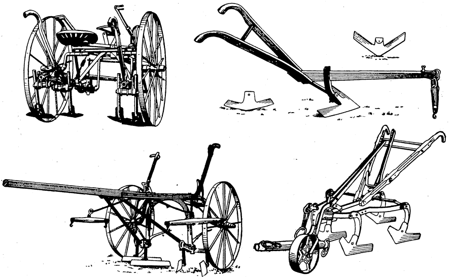
FIG. 22.—Various types of cultivators equipped with knives or sweeps that are effective in cutting off the stems of perennial weeds below the soil surface.
