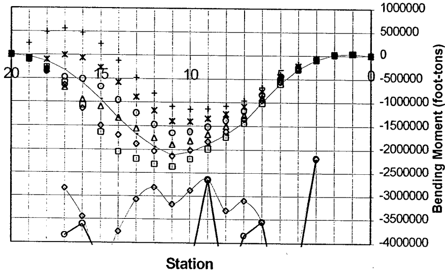
CVN 77 Sagging Bending Moment +10Ktons at stations 15 to 20
