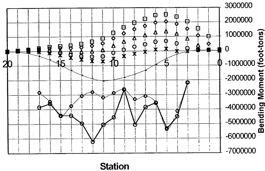
CVN 71 Sagging Bending Moment +11Ktons at stations 0 to 4
