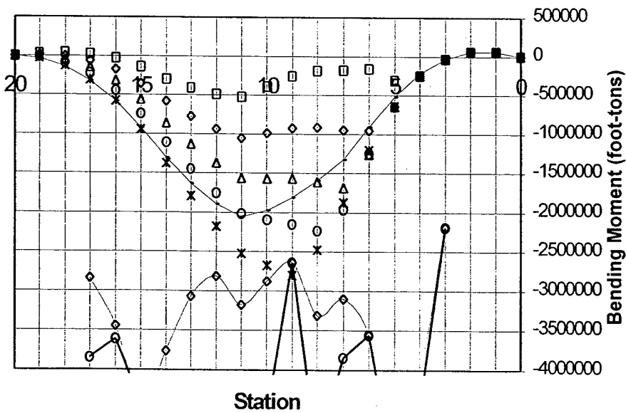
CVN 71 Sagging Bending Moment +15Ktons at stations 5 to 9
