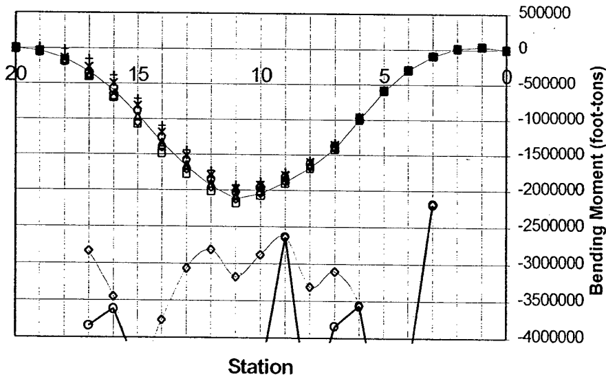
CVN 77 Sagging Bending Moment +2Ktons at stations 15 to 20
