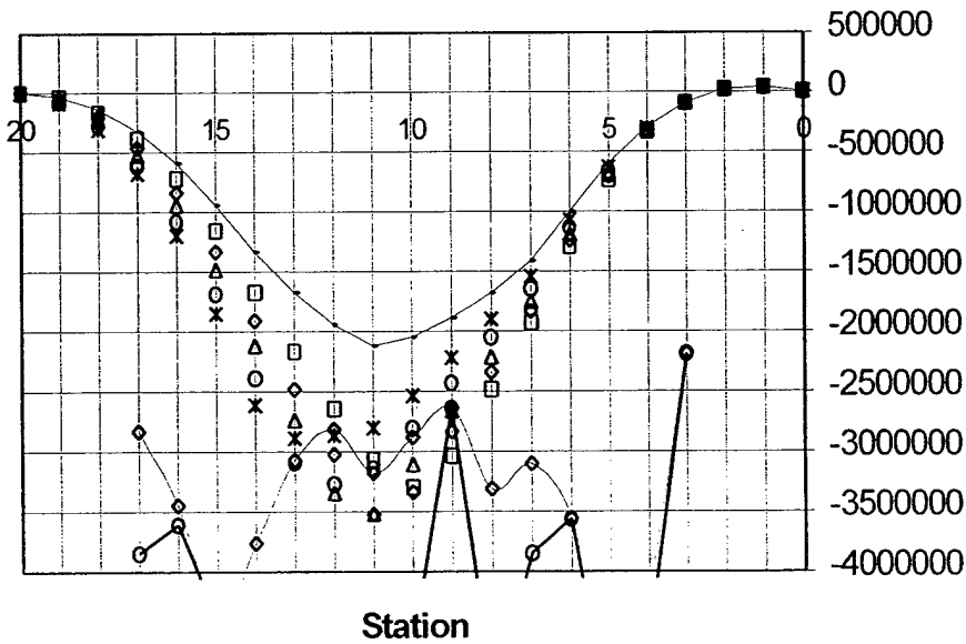
CVN 77 Sagging Bending Moment +15Ktons at stations 10 to 14
