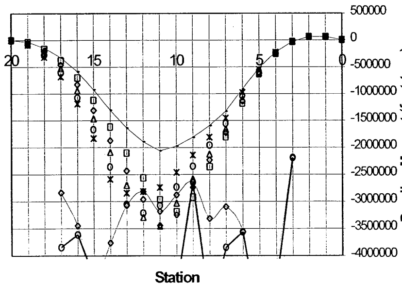
CVN 71 Sagging Bending Moment +15Ktons at stations 10 to 14
