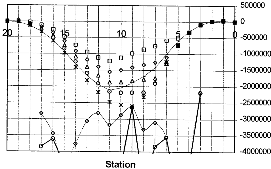
CVN 77 Sagging Bending Moment +10Ktons at stations 5 to 9
