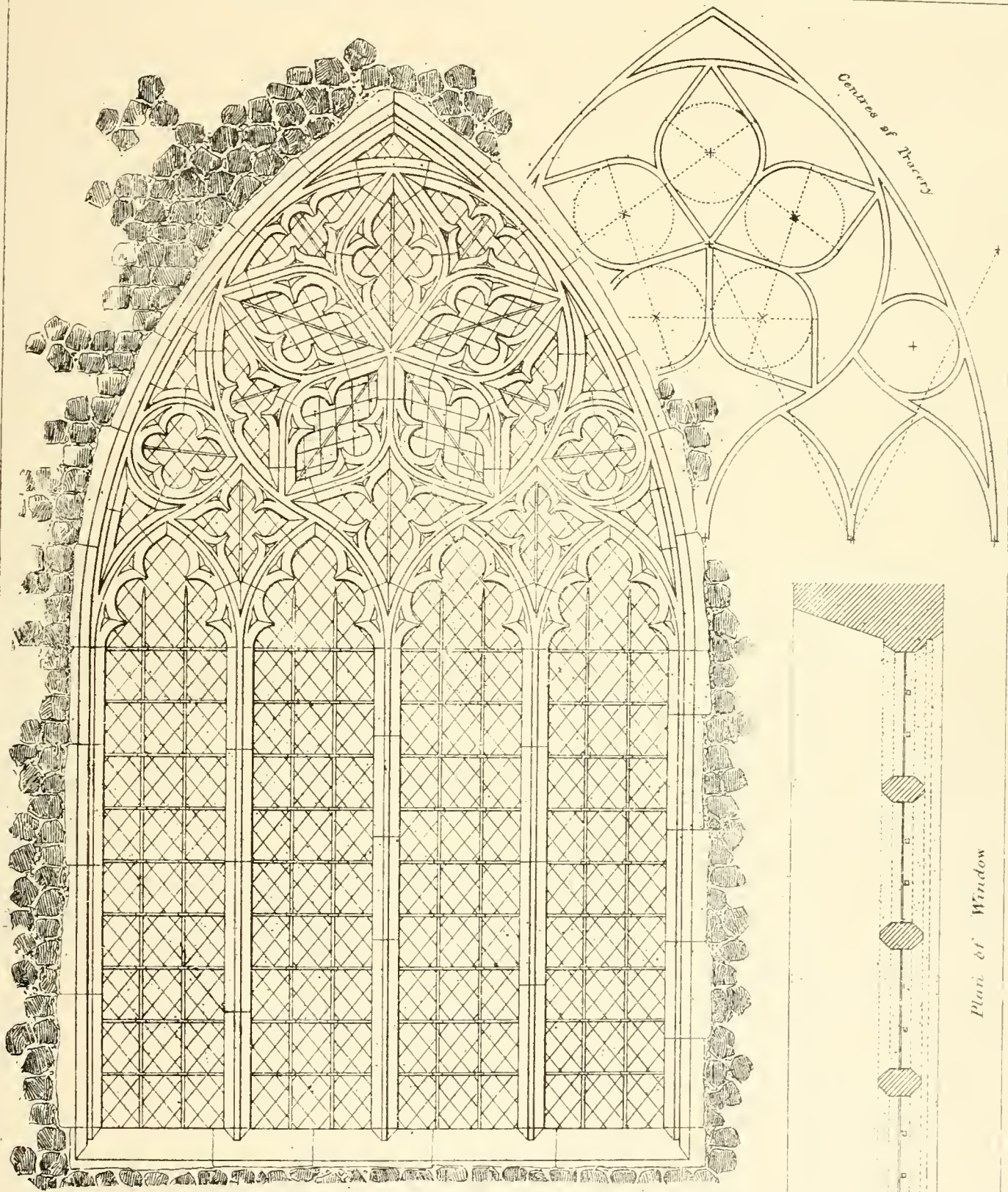
West window from Boughton Aluph Ch. Kent.
