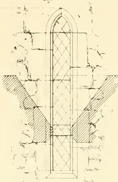
North of Nave Orington Ch. Herts
