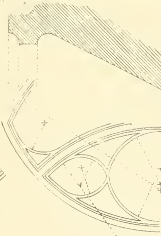
Centres of Tracery
