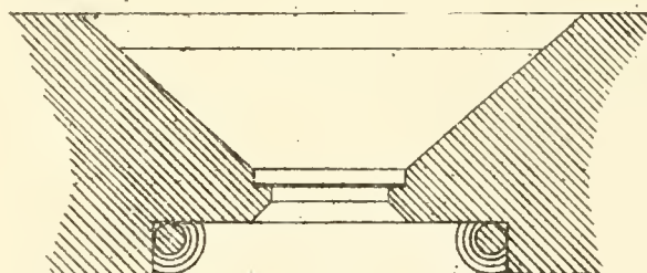
Section of base to shafts 2 m scale.
