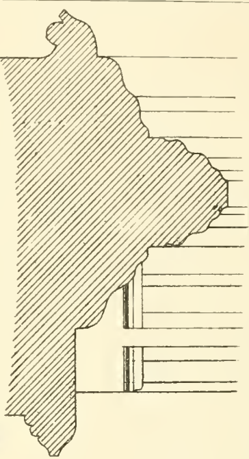
Section of sill 1 st Scale
