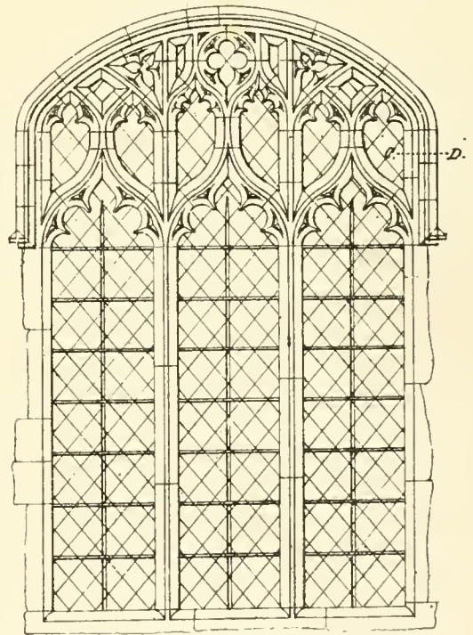
Window South of Nave Rustangles Church Suffolk
