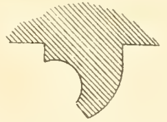
Dripstone. 1 1/2" scale
