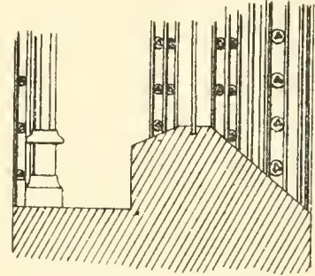
Section of Sill.
