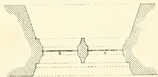
Window N. Aisle of St. Michael's Church, Hertfordshire
