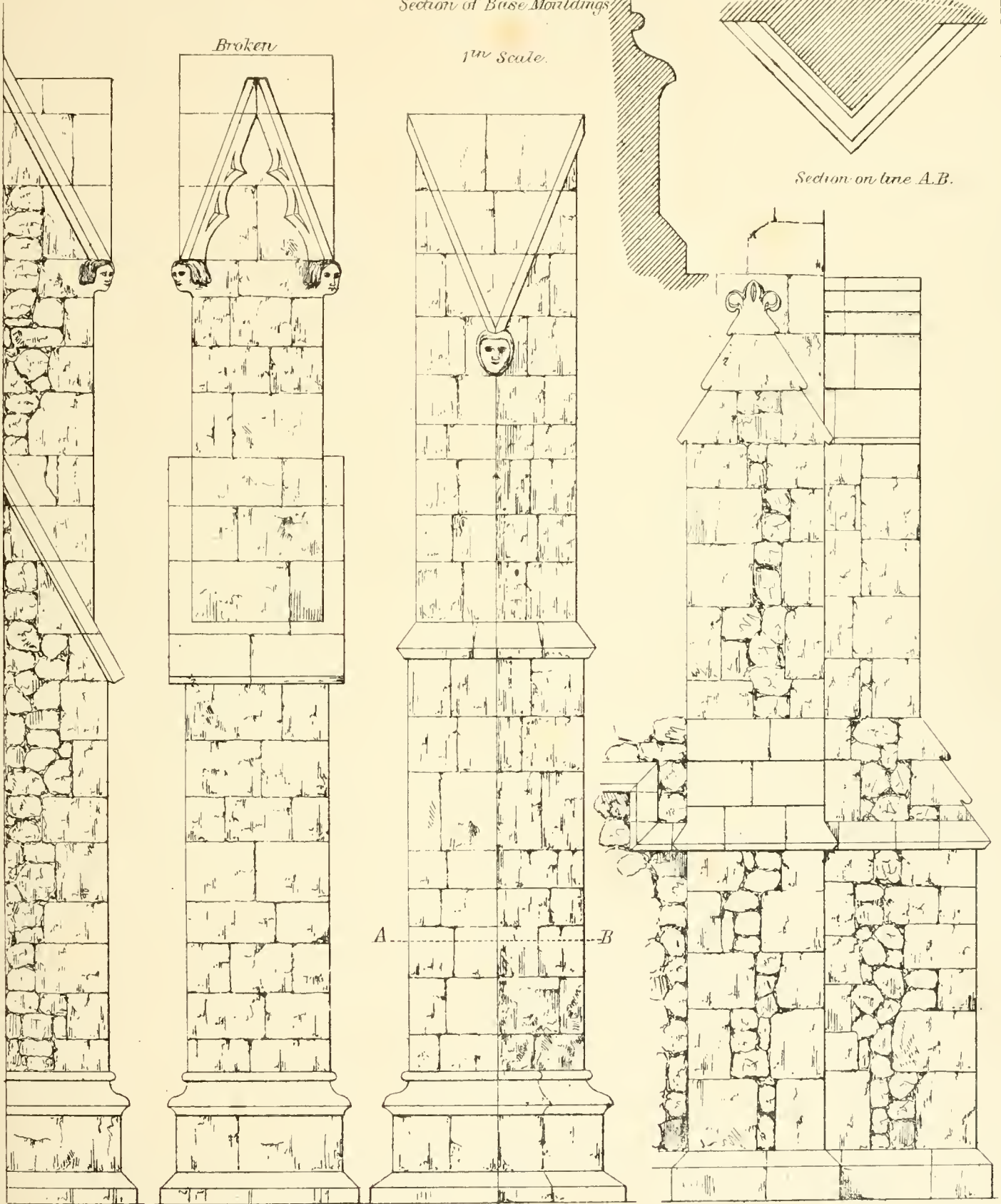
Buttresses from Little Wenham Church, Suffolk
