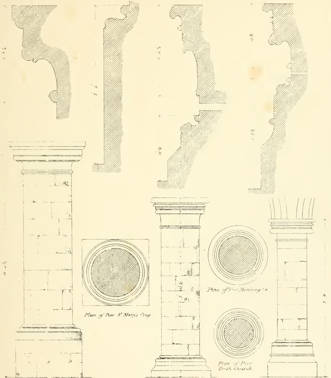
Pier from St. Mary's Cray, Kent.
