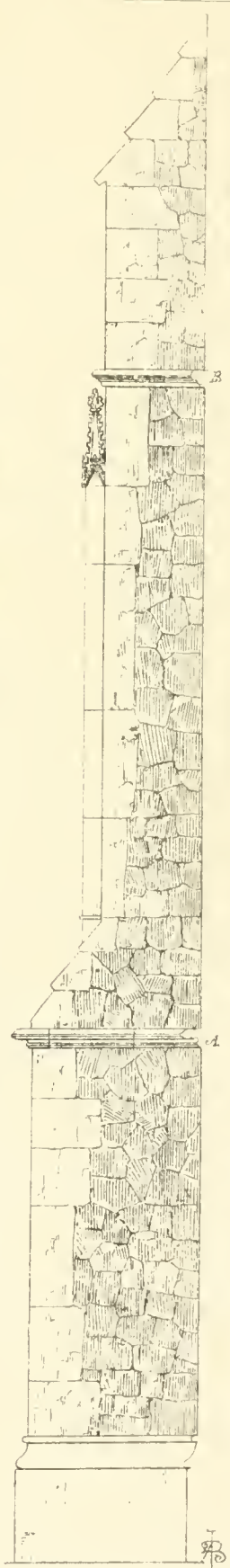
Buttress from Delnabram Ch. Suffolk
