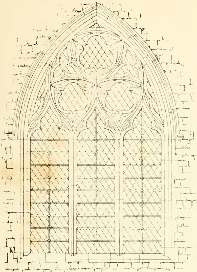
East Window in N. Aisle Northfleet Church Kent
