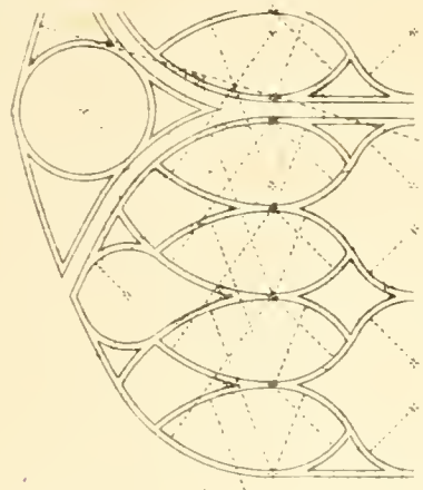
Centres of Tracery
