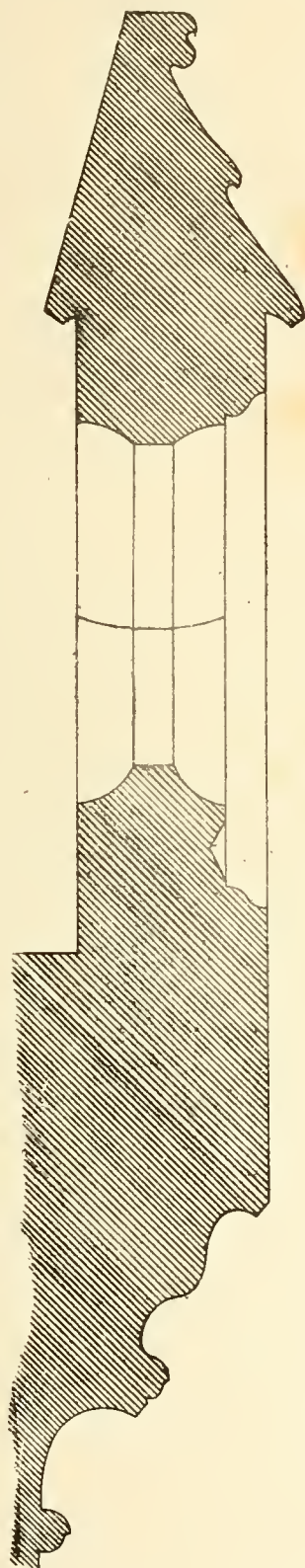
Section of Parapets from Heckington Church
