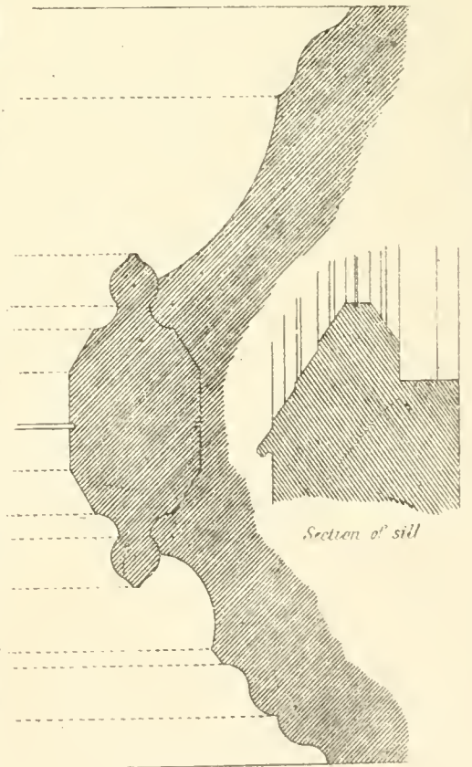
Jamb mouldings 1\frac{1}{2} scale.
