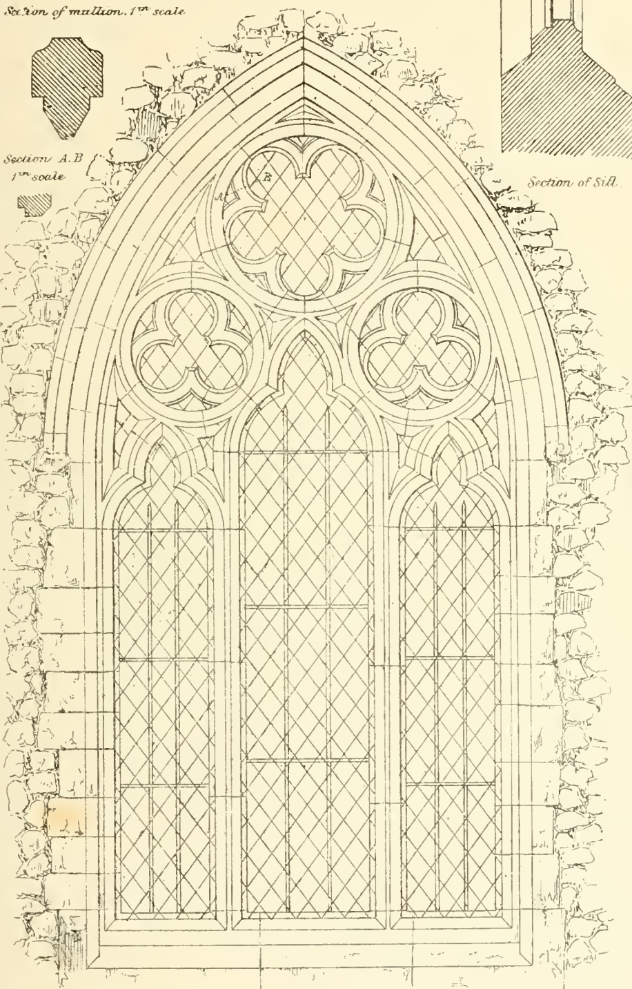
East Window from Chapel, Meopham Ch. Kent.
