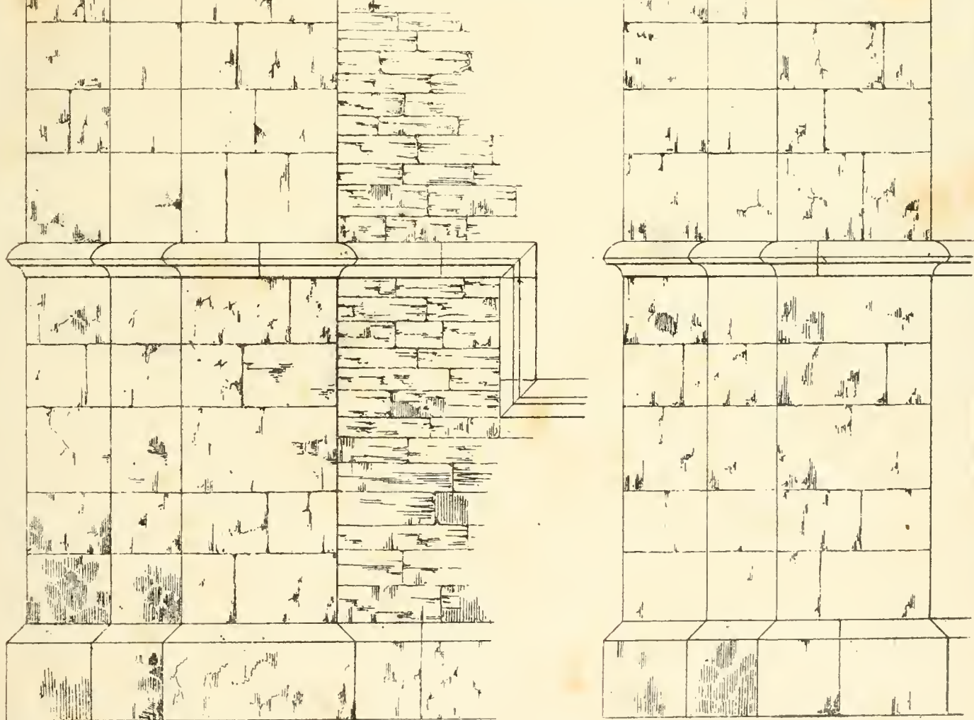
Section on line 00 1/4 full size
