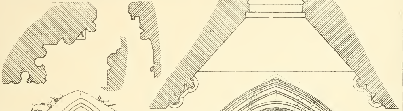
Section of cap, base and arch mold 1/2" Scale.
