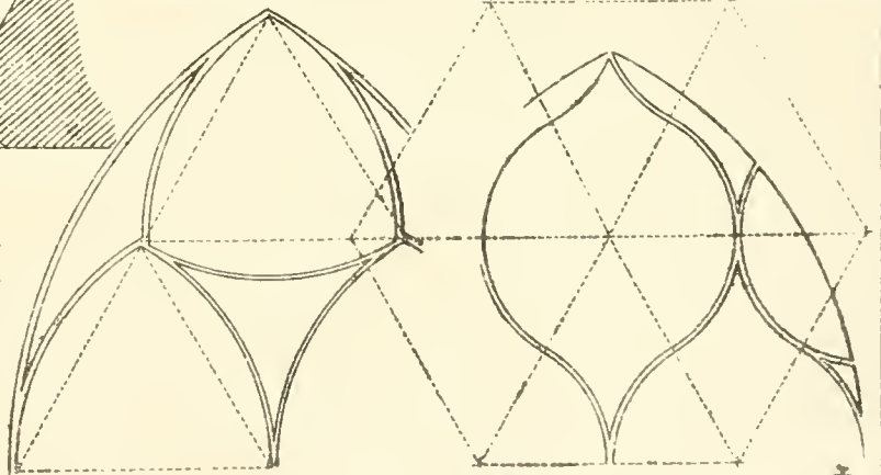
Centres of Tracery
