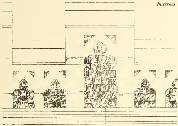
Part of Parapet to an 1/2 w scale
