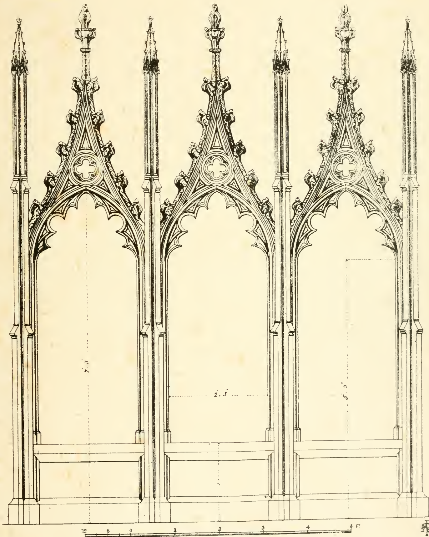
Sedilia in Chapel Cobham Church, Kent.
