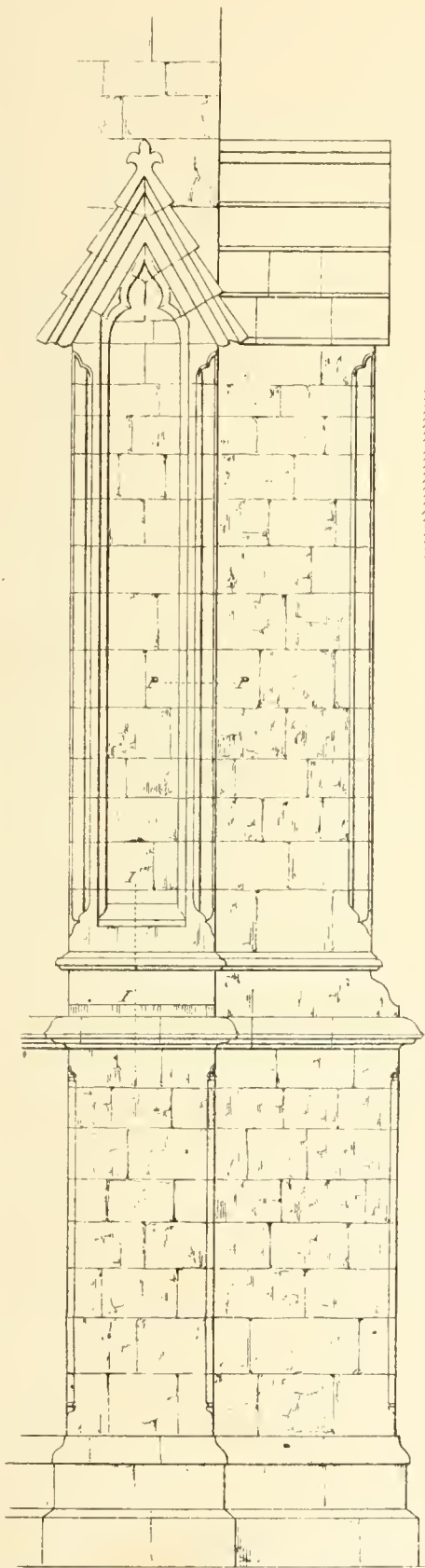
Buttress from Boltisham Ch. Cambridgehire. Scale of
