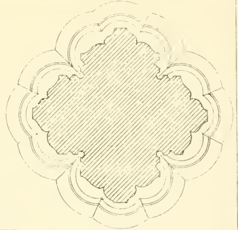
Plan of pier, Trumpington Ch 3/4" scale
