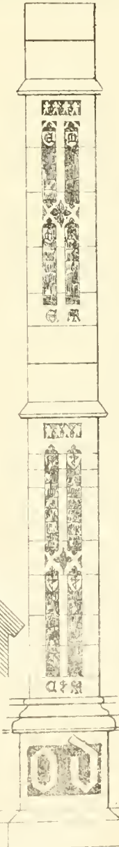
Mouldings 1/4 w scale
