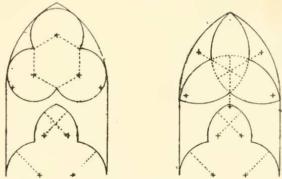
Centres of tracery
