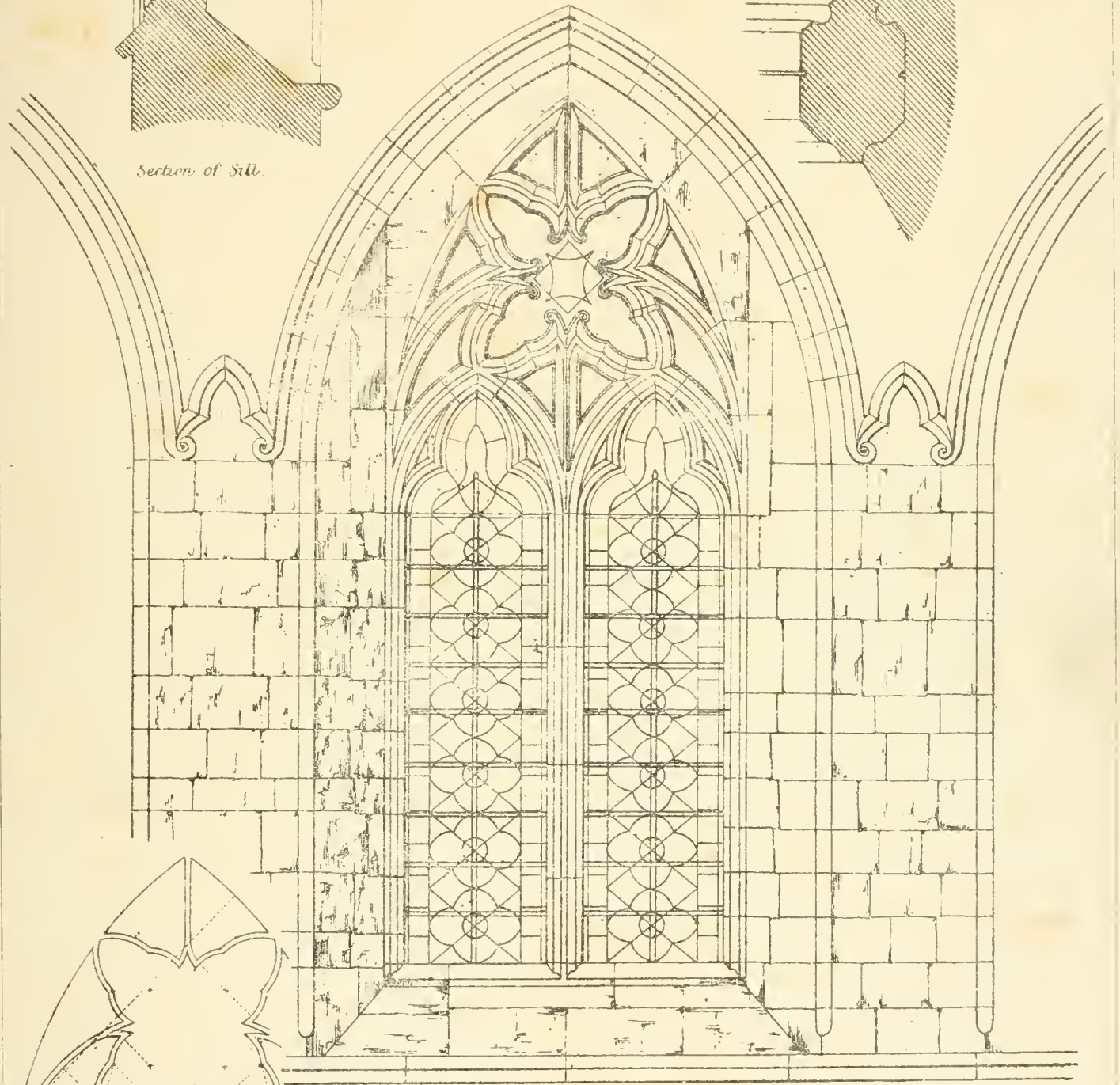
Section of hood mold 1 1/2" Scale.
