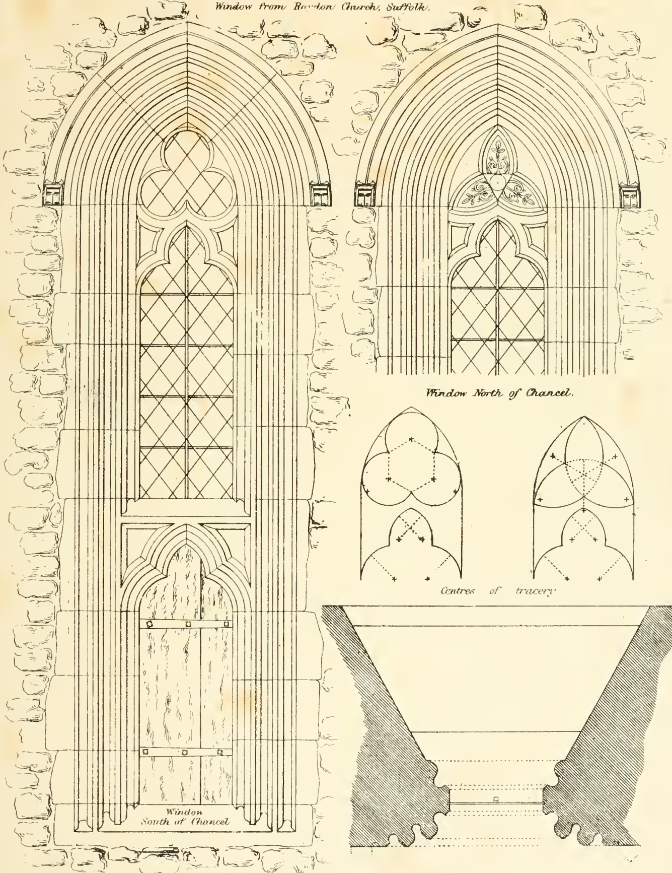
Window from Ravdon Church, Suffolk.
