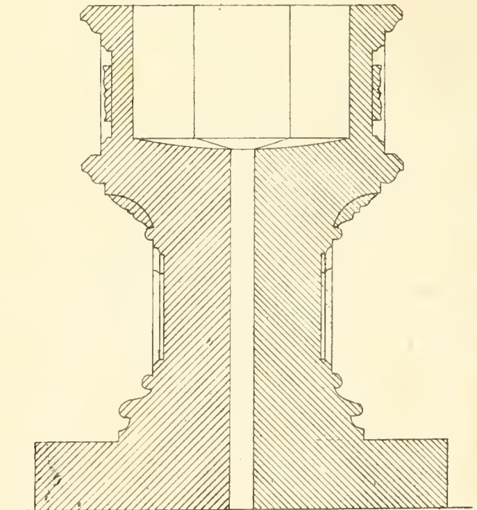
Font in Glymping Church, Sussex.
