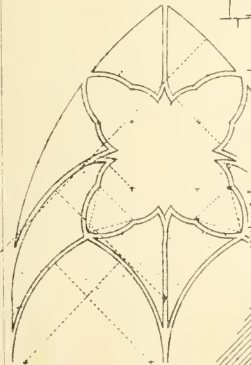
Centres of Tracery
