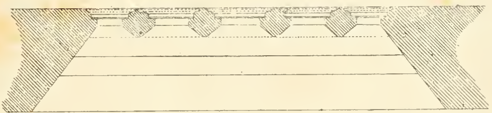
Section of archstone 1/4 th scale
