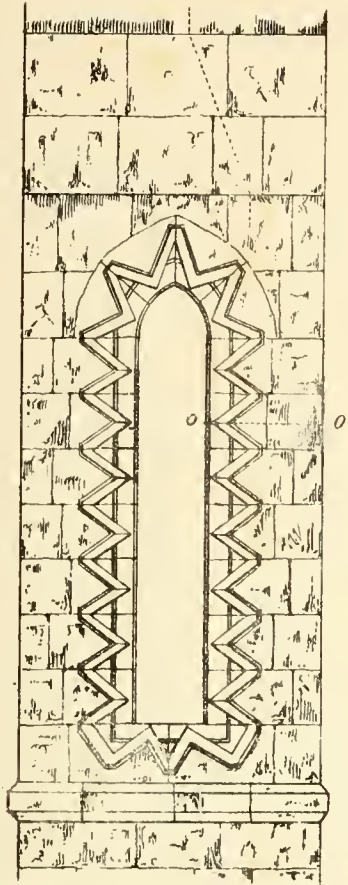
Plan and Elevation of Window in Buttress Climping Ch. Sussex.
