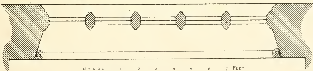
East Window of Chancel from Trumpington Church, Cambridgeshire.
