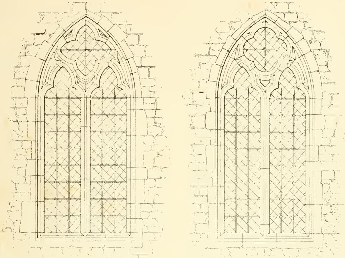
Windows in South aisle Northwell Church Kent
