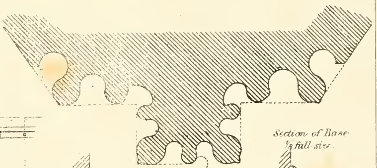
Section of cap 1/3 full size
