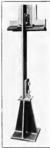
COLUMN STRONGLY BOLTED AND CLAMPED TO BASE AND IRON SILL
