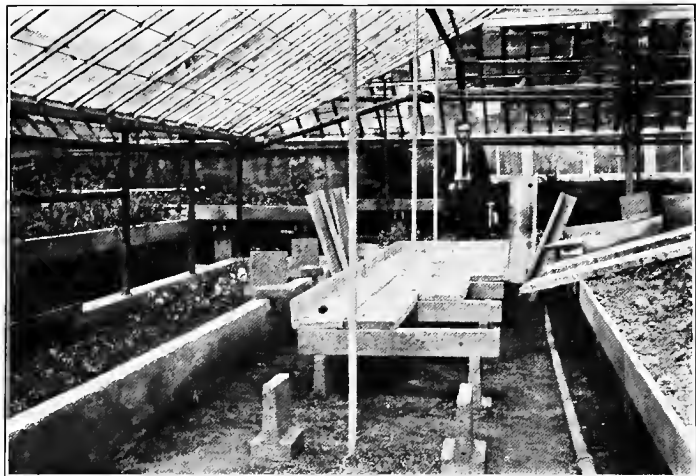
McCASLAN'S SECTIONAL CONCRETE BENCH IN SECTIONAL SLABS
