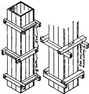
MOLDS FOR CEMENT POSTS (See text)
