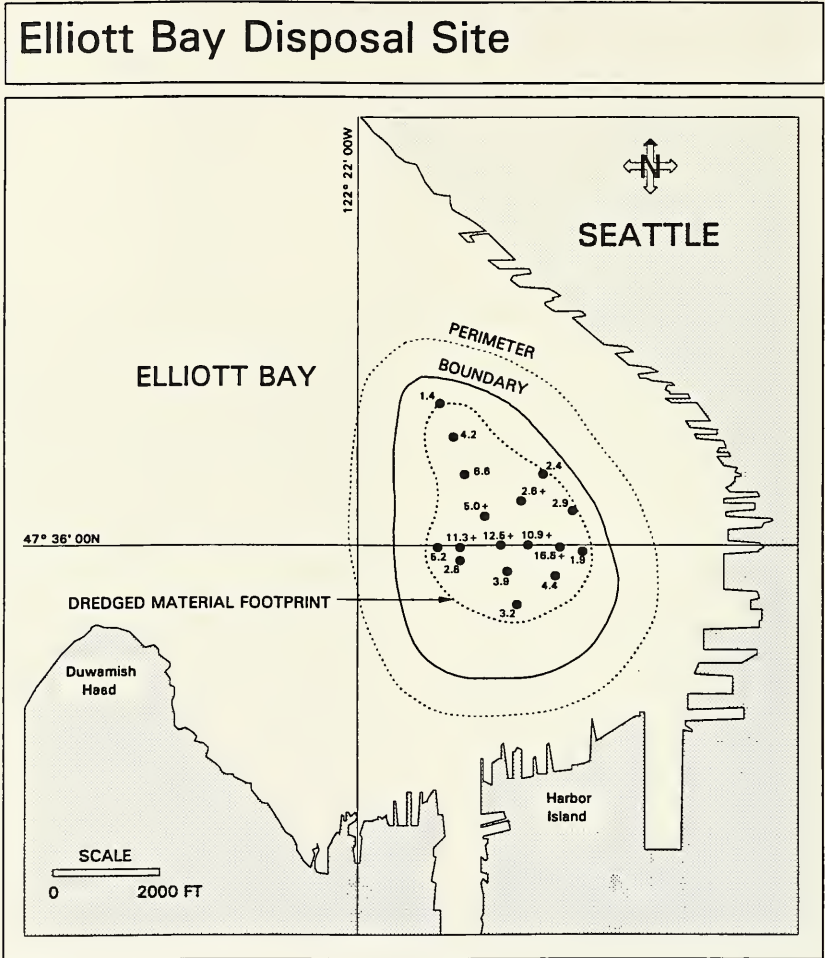
Figure 3-7. The distribution of dredged material (cm) at the Elliott Bay disposal site as detected by REMOTS®. The solid line is the site boundary; the dashed line is the site perimeter. The "+" indicates dredged material greater than penetration.
