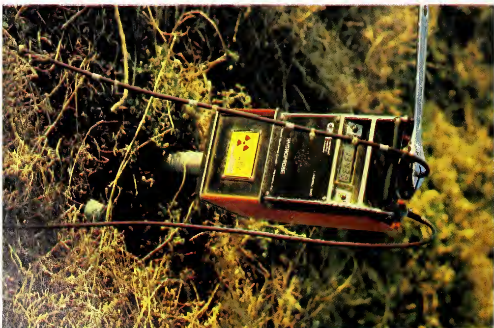
Figure 30. Neutron attenuation probe in an access tube.
