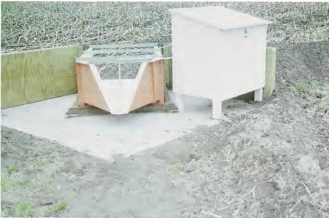
Figure 24. Surface water runoff instrumentation for a vadose zone monitoring site.
