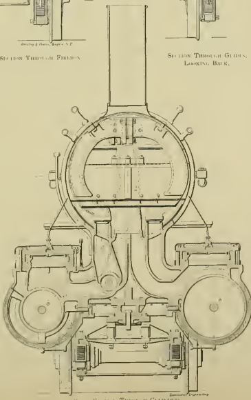
CROSS SECTION THROUGH CYLINDERS.
