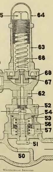
PLATE 6. WESTINGHOUSE IMPROVED.
