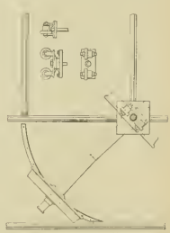
SCHEMATIC FOR TURN-TABLE IN WHEEL SHOP.
