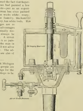
CORY'S LUBRICATOR, SECTIONAL VIEW.
