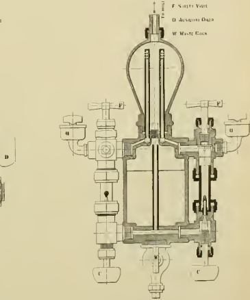
SECTIONAL FRONT VIEW "NATHAN"
