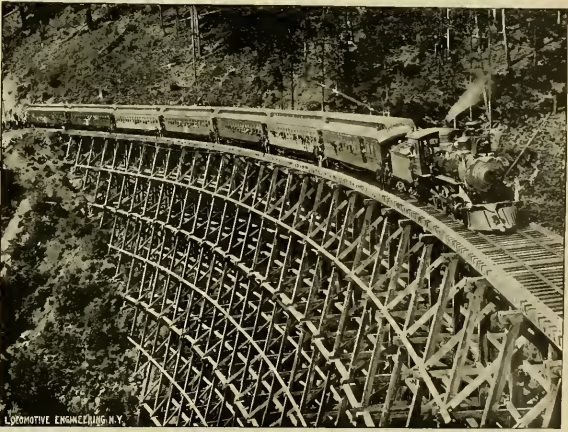
IN ARDUS CASON, BRITISH COLUMBIA—BRIDGE 225 FEET HIGH, ON ENGLISH & NANAIMO RAILWAY.
