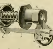
CHUCK PACKING FORMER AND SPRING COMPRESSOR
