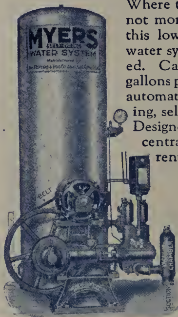
Fig. 2510 — Myers Shallow Well Water System
