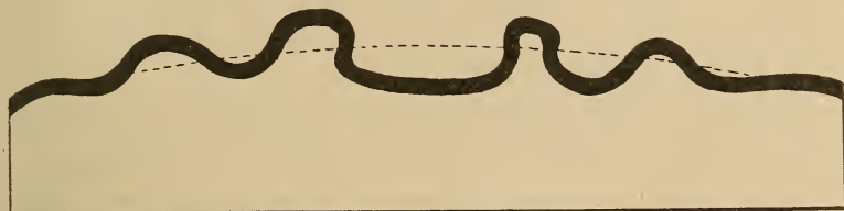
FIG. 2. Cordilleran anticlinorium, with unfolded center.
