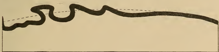
FIG. 3. Orographic flexure, with overturned fold.
