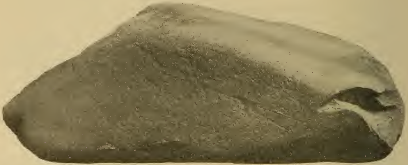
FIG. 10.—Glaciated quartzite boulder, from the tillite at the inner end of the Altenfjord. Entire surface also with fine slickensided strata due to the Caledonian deformation. One half natural size.
