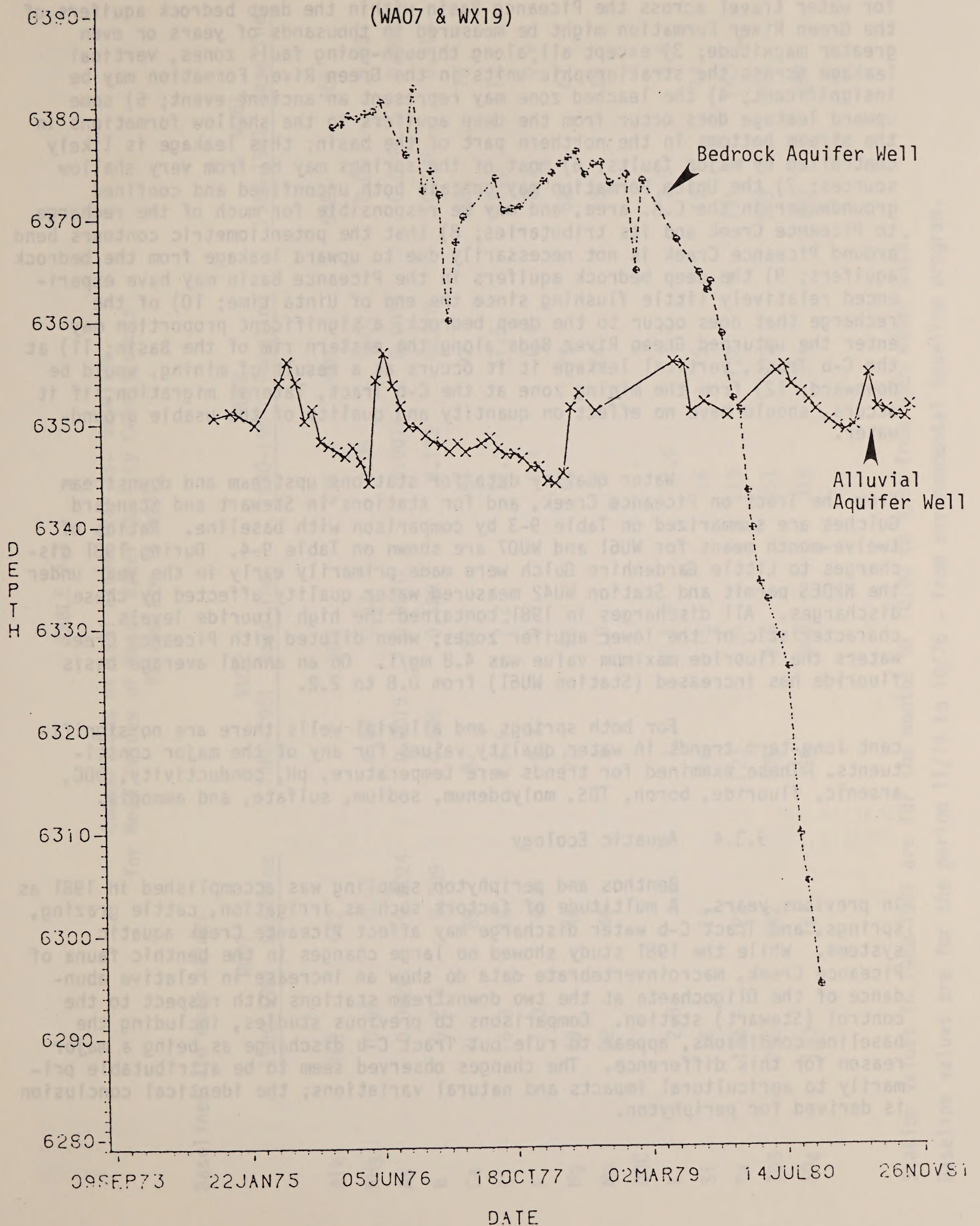
Figure 9-9 Comparison of Water Levels in Cb Well Pairs during Shaft Development
