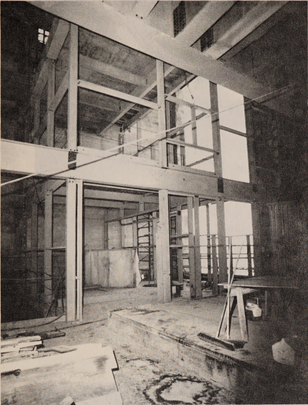
Figure 4-12. Upper and lower power floors in the production headframe. (October 1981)
