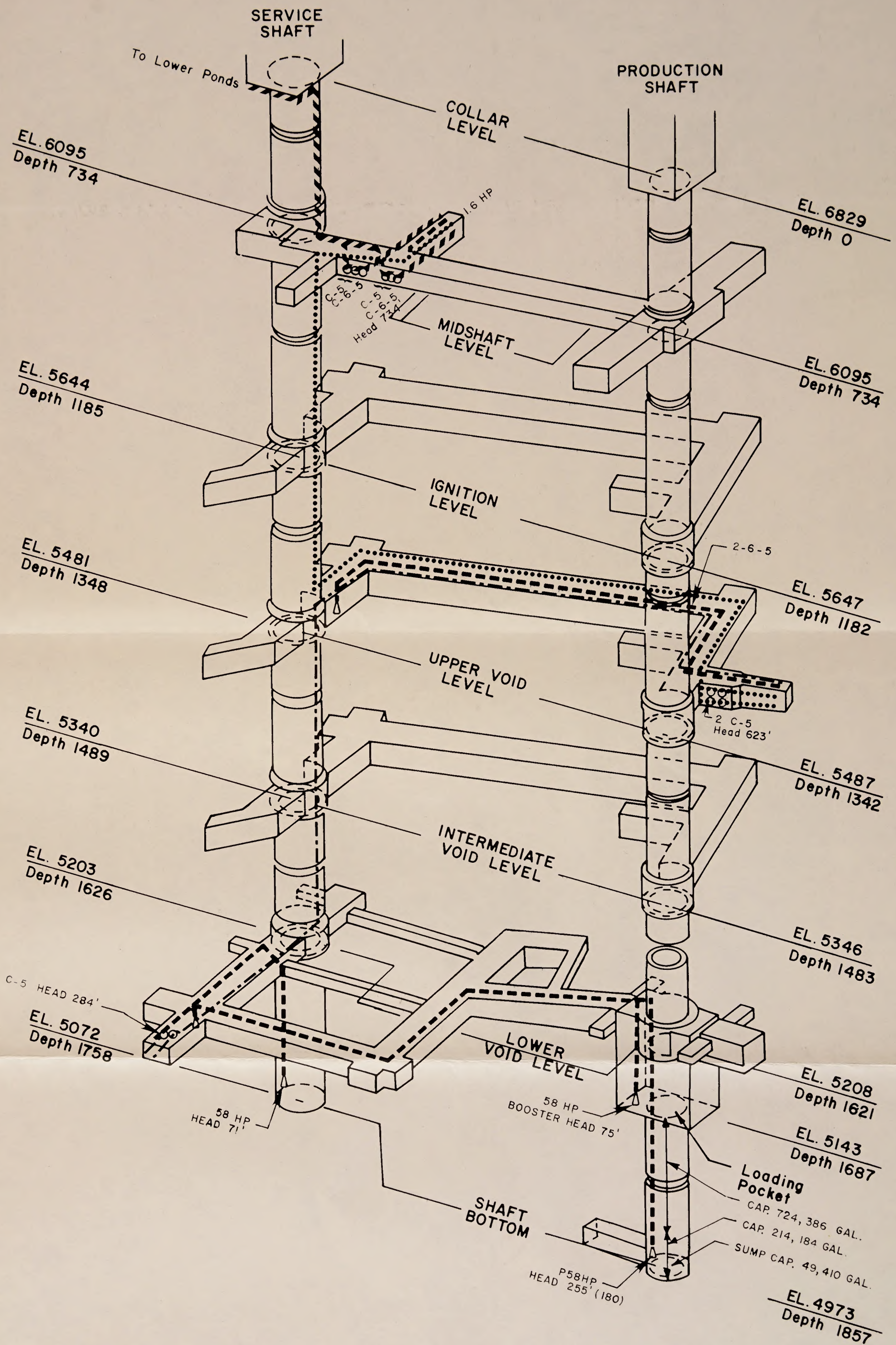
Figure 4-37 The production and service shaft station development illustrating the dewatering pumping system.
