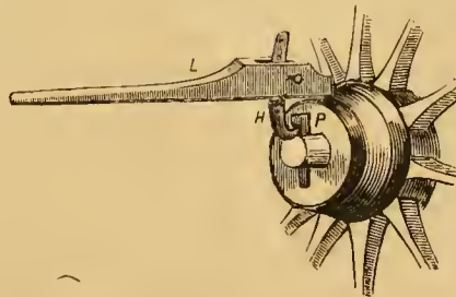
A Linch-Pin Extractor.
