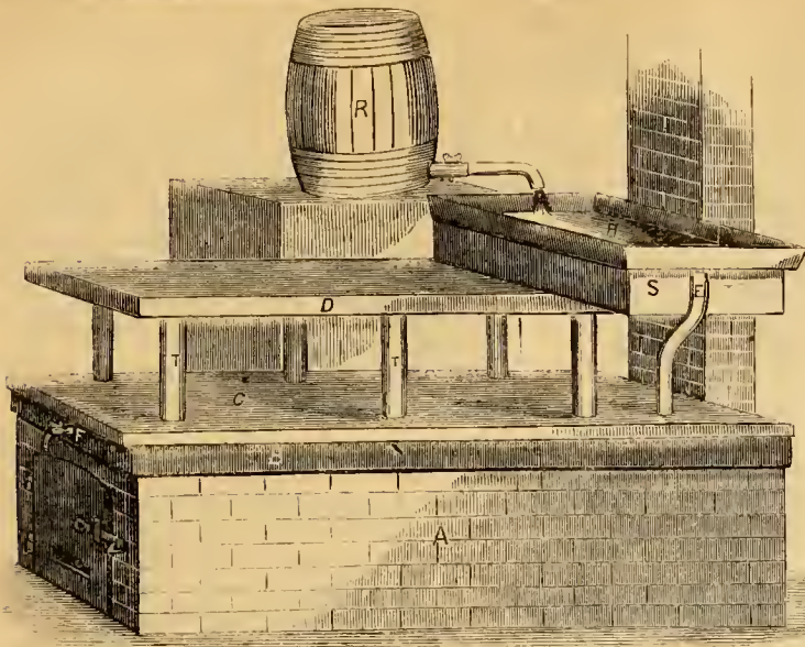
Miles' Improved Sap Boiler.
