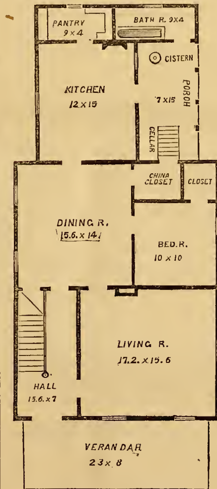
Fig. 3.—PLAN OF FIRST STORY.
