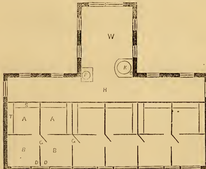
Fig. 3.—GROUND PLAN OF PIGGERY.
