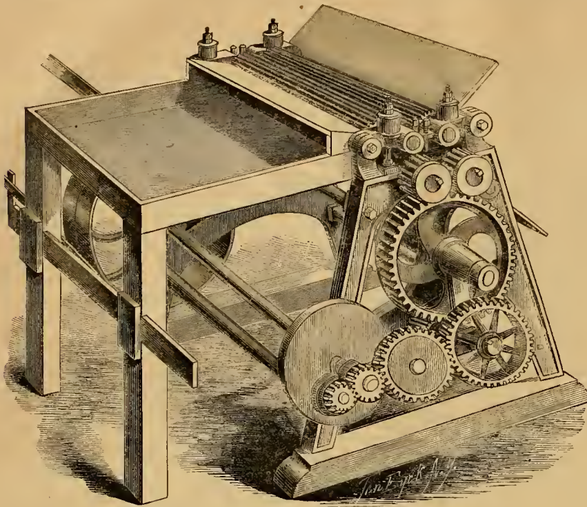
MALLORY &amp; SANFORD'S IMPROVED FLAX BRAKE.
