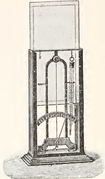
Fig. 3. Haarhygrometer.
