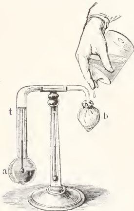
Fig. 2. Daniell'sches Hygrometer.
