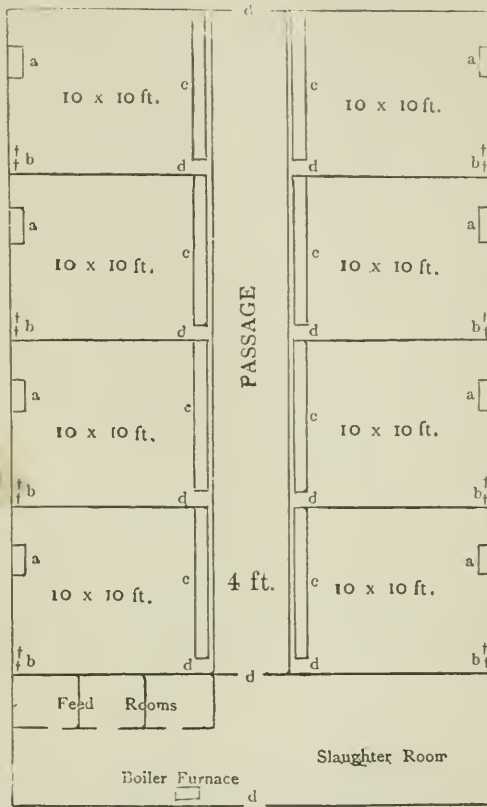
GROUND PLAN OF PIGGERY.
