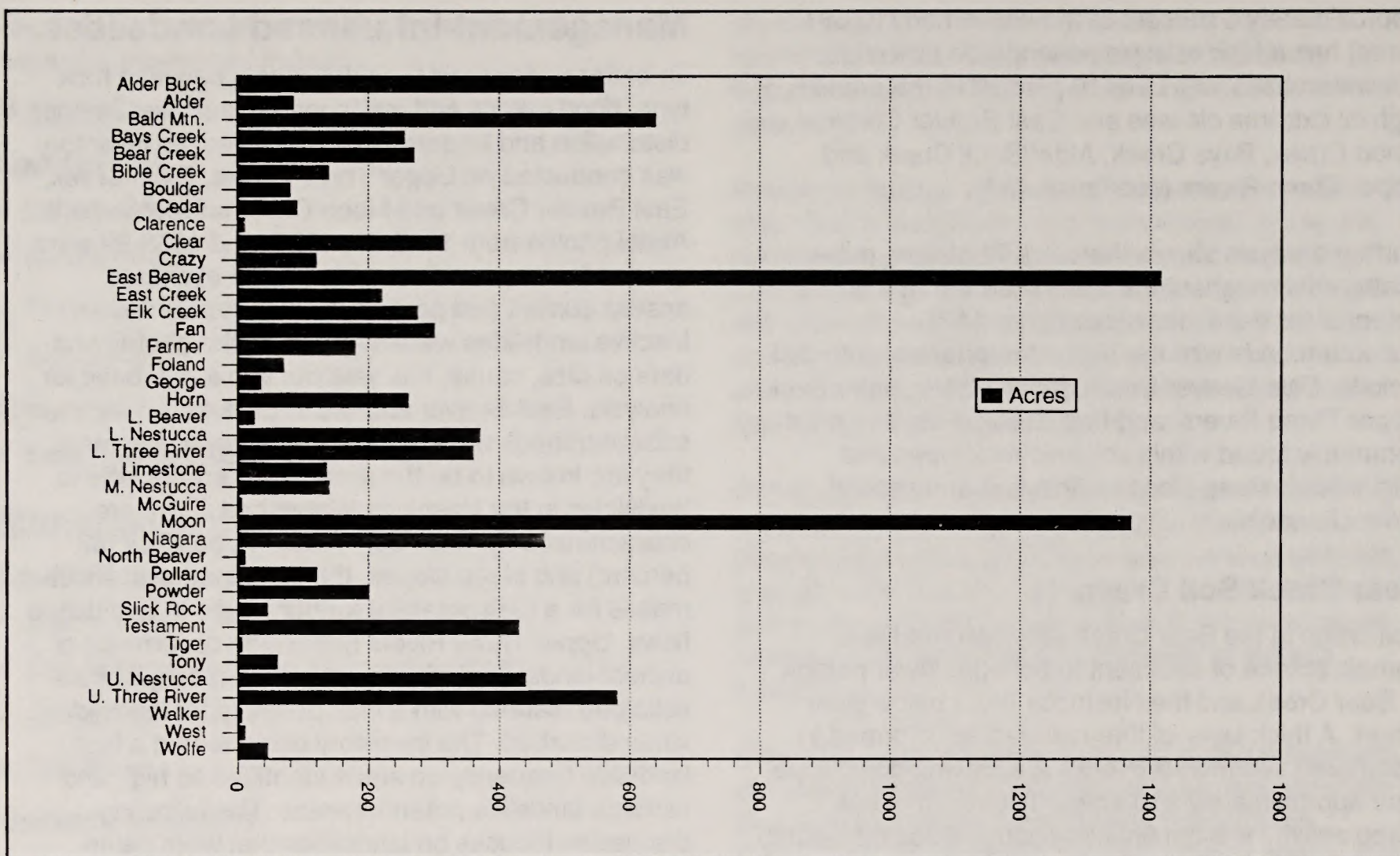
Figure 4A1 High and Extreme Debris Slide Potential
