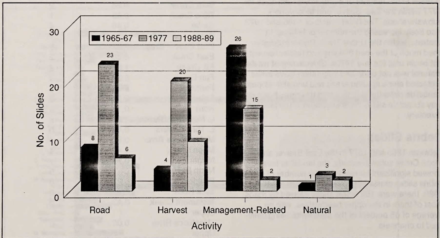
Figure 4A4 East Beaver and Moon Creek Active Debris Slide by Activity and Photo Year Debris flows caused by management activities increased after 1972 storm event. Management-related debris slides are associated with road and harvest activities, however, a probable cause was not evident on aerial photos.
