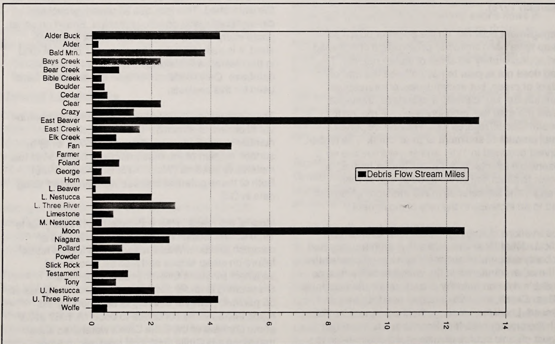
Figure 4A2 Debris Flow Potential by Subwatershed
