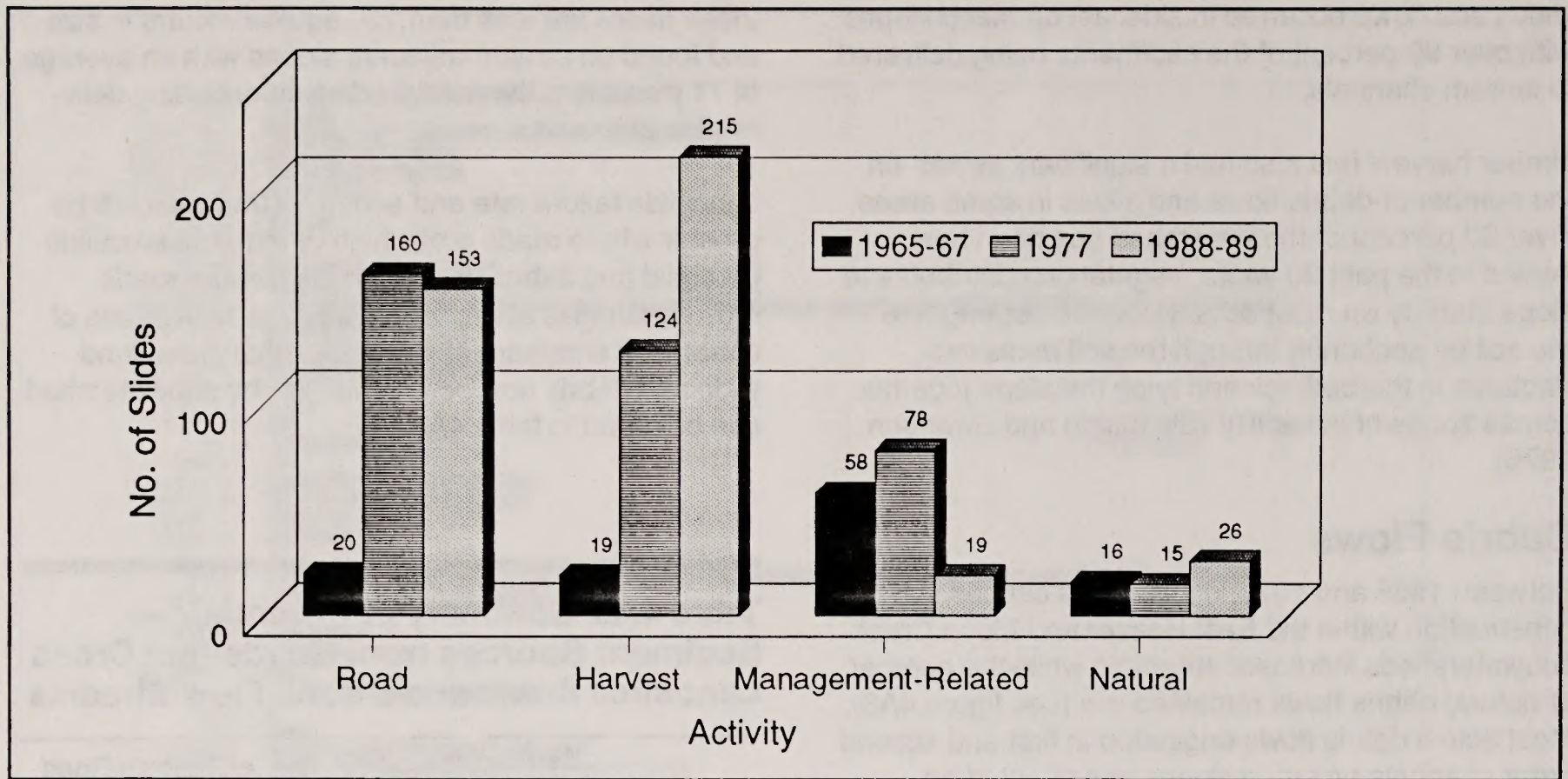
Figure 4A3 East Beaver and Moon Creek Active Debris Slide by Activity and Photo Year Management-related debris slides are associated with road and harvest activities, however, a probable cause was not evident on aerial photos.
