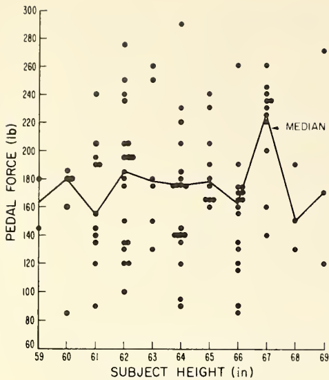
PEDAL FORCE vs SUBJECT HEIGHT FOR APPLICATION 2
