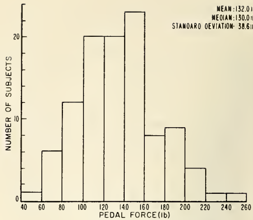
PEDAL FORCE HISTOGRAM FOR APPLICATION 4
