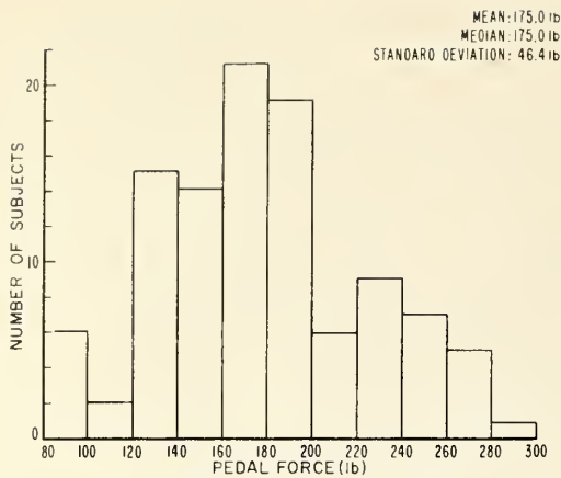
PEDAL FORCE HISTOGRAM FOR APPLICATION 2
