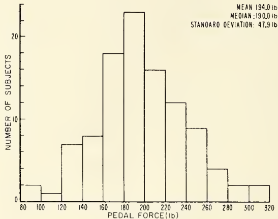
PEDAL FORCE HISTOGRAM FOR APPLICATION 6
