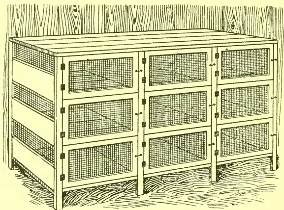
Practical Type of Indoor Hutch.
