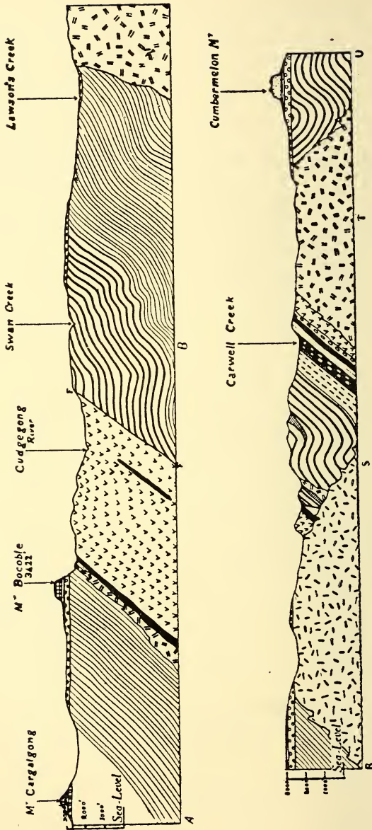
Fig. 1.—Sections across the Cudgegong district. Geological units indicated as on map, Plate VIII.
