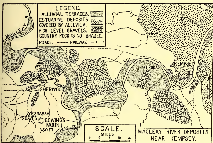
Fig. 2.—Macleay River Deposits near Kempsey.
