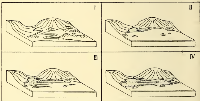
Fig. 3.—Stages in the Evolution of the Lower Macleay Plain.
