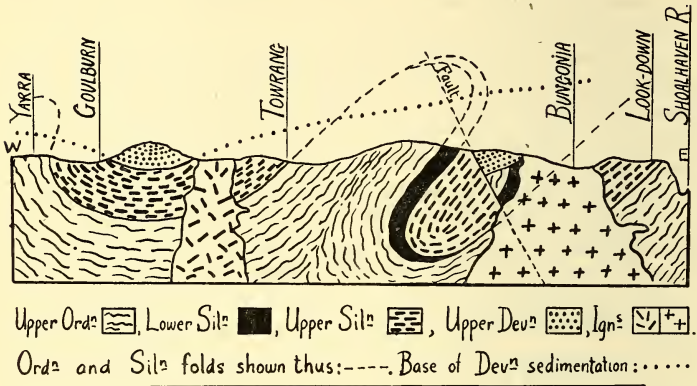
Fig. 1.—Sketch-section to show the geological structure in the Goulburn-Bungonia area.
