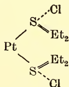
\beta dichloride.
