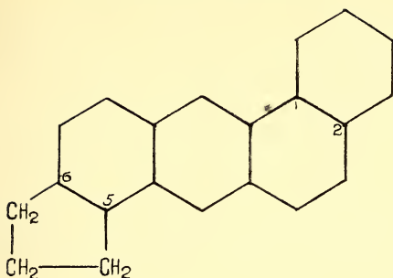
5:6-cyclopenteno-1:2-benzanthracene, and
