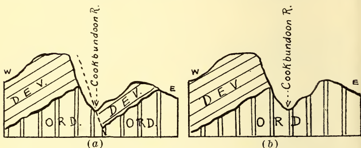
Fig. 1. Alternative Interpretations of the Cookbundoon Scarp.
