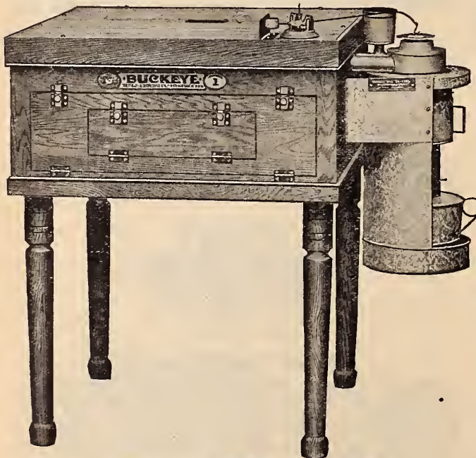
Buckeye No. 1, Standard 110—Egg Incubator
