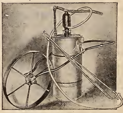
Auto No. 40 Portable Sprayer
