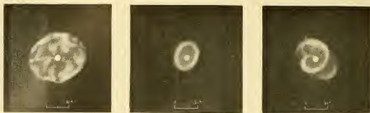
FIG. 1. (a) N.G.C. 1501. (b) N.G.C. 418. (c) N.G.C. 6543. Planetary Nebulae. Composite drawings by Curtis from his photographs with the Crossley Reflector of the Lick Observatory.
