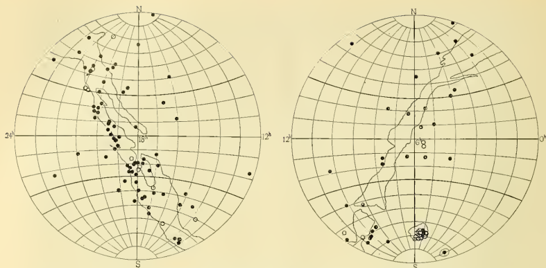
FIG. 11. Distribution of Planetary and Irregular Bright-line Nebulae.
