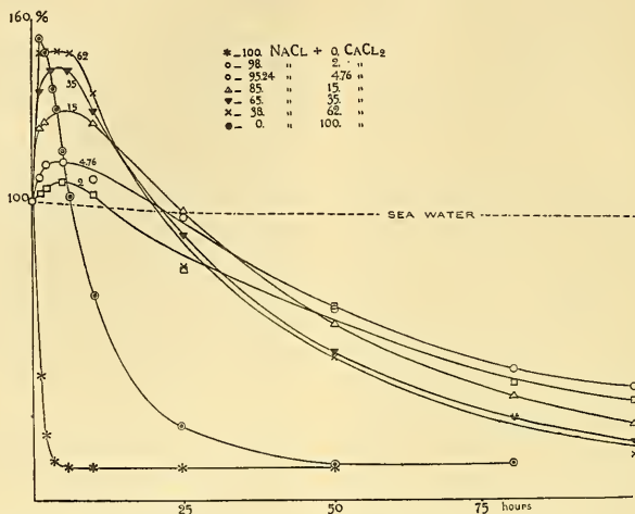
FIG. 1. Curves of electrical resistance of Laminaria in NaCl .52M, in CaCl 2 .278M, and in mixtures of these (the figures show the molecular percent. of CaCl 2 in the mixture).
