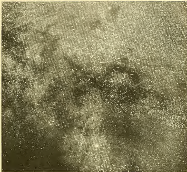
FIG. 18. The Milky Way in Ophiuchus showing apparent absorption or obstruction effects; photographed by Barnard with the 10-inch Bruce telescope of the Yerkes Observatory.
