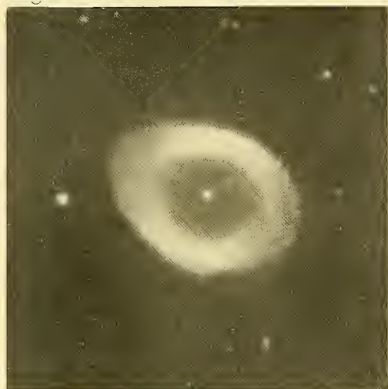
FIG. 33. The Ring Nebula in Lyra, photographed by Curtis with the Crossley Reflector of the Lick Observatory.
