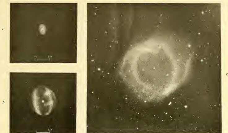
FIG. 10. Planetary Nebulae. (a) and (b) are composite drawings from photographs, and (c) is a direct copy of a photograph, made by Curtis with the Crossley Reflector of the Lick Observatory.
