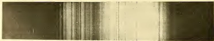
FIG. 35. The Spectrum of Gamma Cassiopeia, Henry Draper Memorial, Harvard College Observatory.
