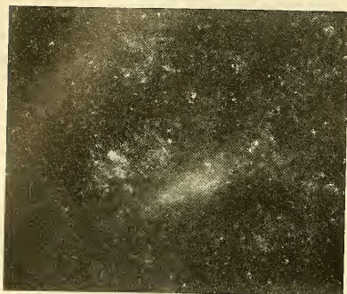
FIG. 22. The Greater Magellanic Cloud, photographed by Bailey, at the Arequipa, Peru, station of the Harvard College Observatory.
