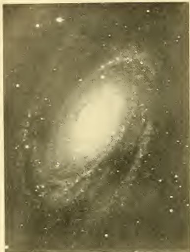
FIG. 4. Spiral Nebula Messier 81, photographed by Keeler with the Crossley Reflector of the Lick Observatory.
