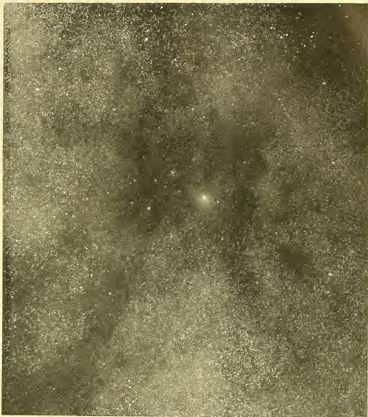
FIG. 37. The Milky Way, photographed by Barnard with the Bruce 10-inch telescope of the Yerkes Observatory.
