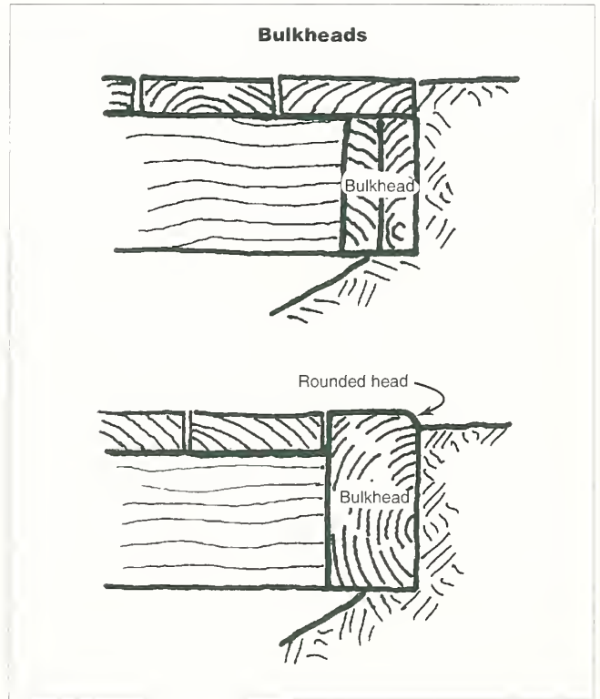
Figure 66—Bulkheads serve as retaining walls to support the earth, and they protect the stringers from rot and insect damage. Here are two different ways to install them.
