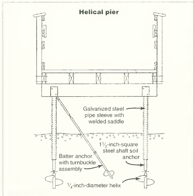
Figure 41—Typical helical pier assembly.
