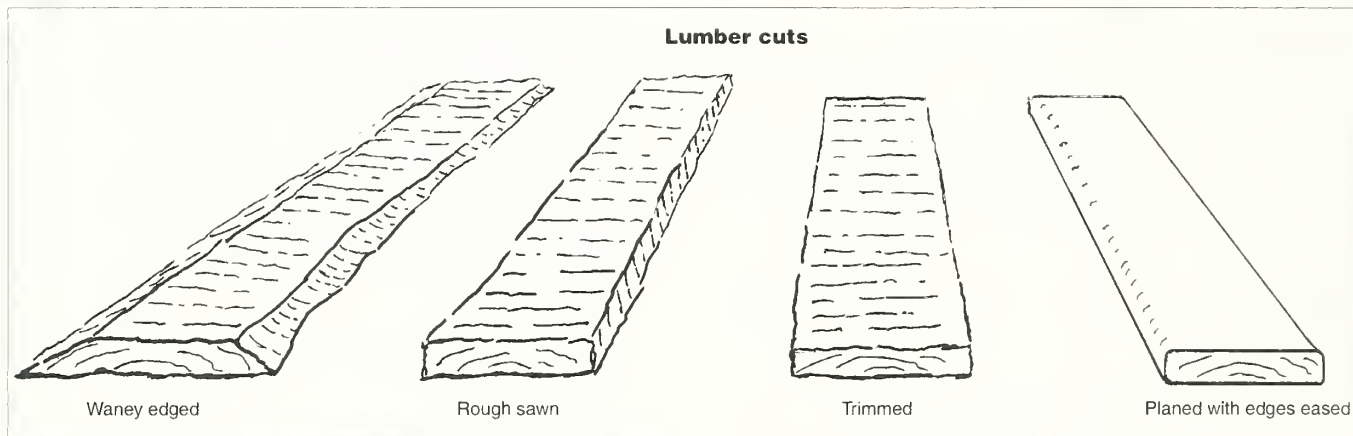
Figure 68—Lumber terminology.
