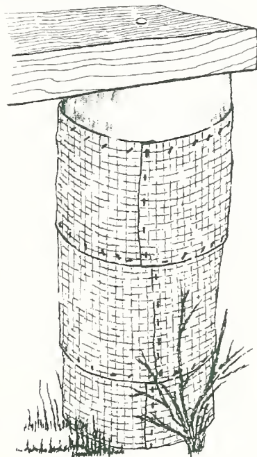
Figure 43—Hardware cloth stapled around piles helps discourage beavers.
