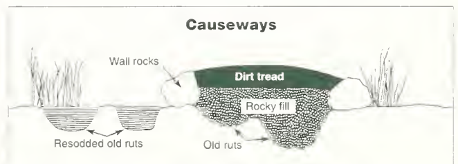
Figure 18—Causeways create an elevated, hardened tread across seasonally wet areas.
