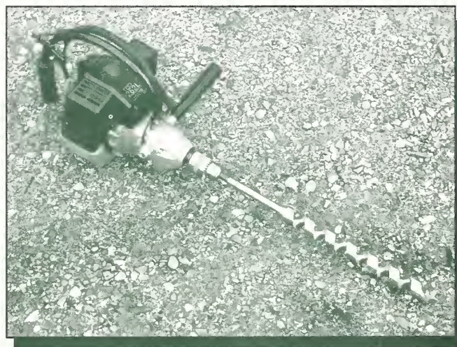
Figure 85—Gasoline-powered drills are great for backcountry work if regulations allow their use.
