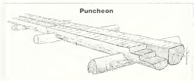
Figure 45—A rustic type of puncheon with stringers and tread logs.
