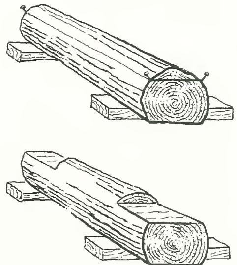
Figure 96—Use this procedure when a second flat surface must be parallel to the first.
