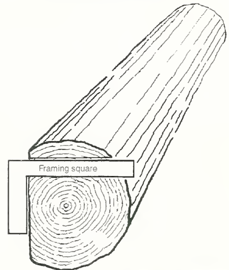
Figure 95—Use a framing square to mark a perpendicular cut.
