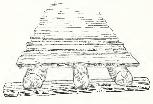
Figure 46—A second type of puncheon with stringers and decking.
