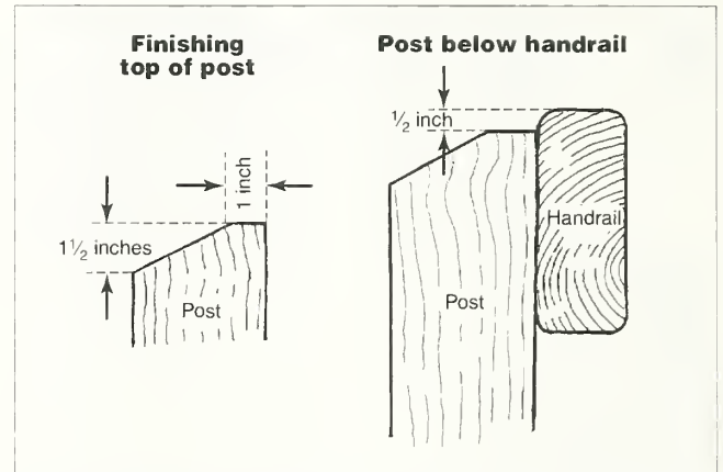
Figures 59 and 60—Cut the top of the post at an angle, but leave 1-inch flat on the inside edge. The post should not extend above the top of the handrail.
