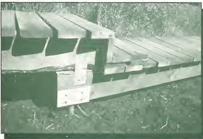
Figure 38—A helical pile was used for this boardwalk. Stringers are attached directly to the beam saddle, helping to keep the boardwalk close to the ground.
