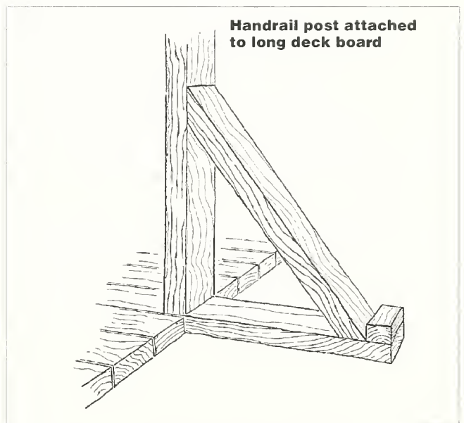
Figure 57—Attaching the handrail post directly to the decking requires long deck pieces to support an angle brace.
