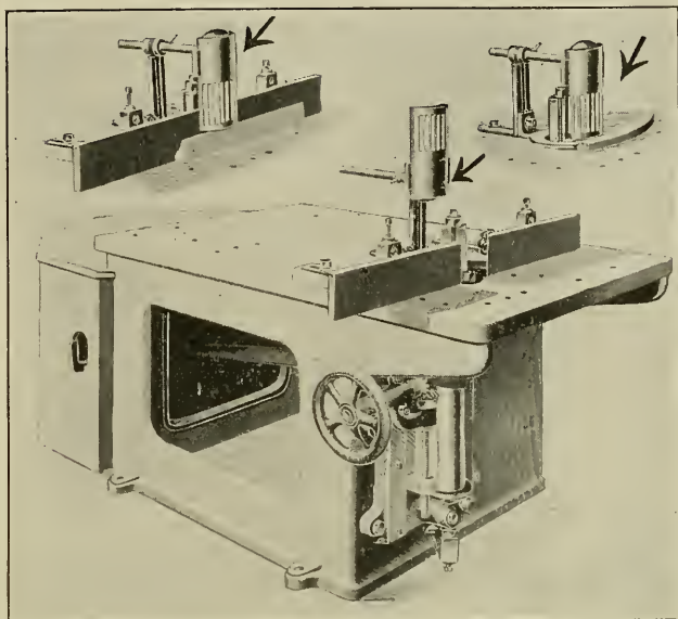
Fig. 183. Campbell Guard for Shaper.
