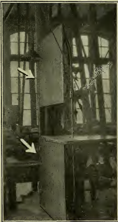
Fig. 141. Guards for Band Saw Wheels.
