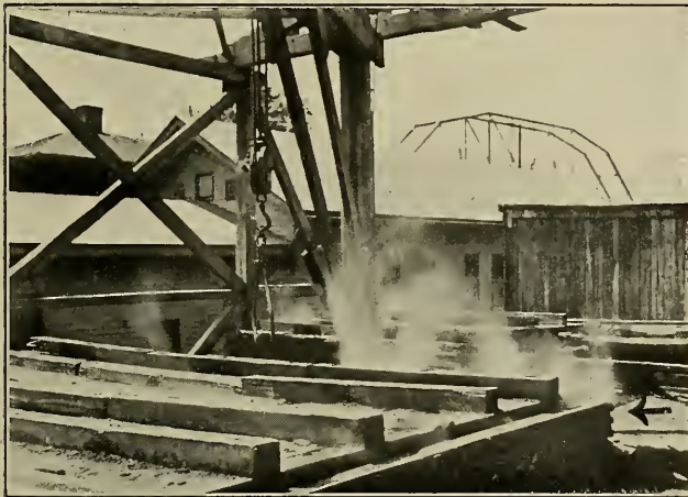
Fig. 247. Vat with Built-up Sides.
