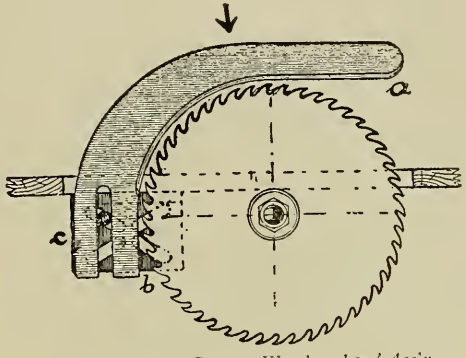
Fig. 86. Extended Splitter.
