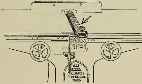
Fig 151. "Wills" Jointer Guard.
