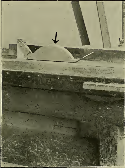
Courtesy of Fairbanks, Morse & Co. Fig. 109. McKee Saw Guard, Attached to Splitter.
