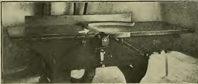
Fig. 163. Finger Guard for Jointer.
