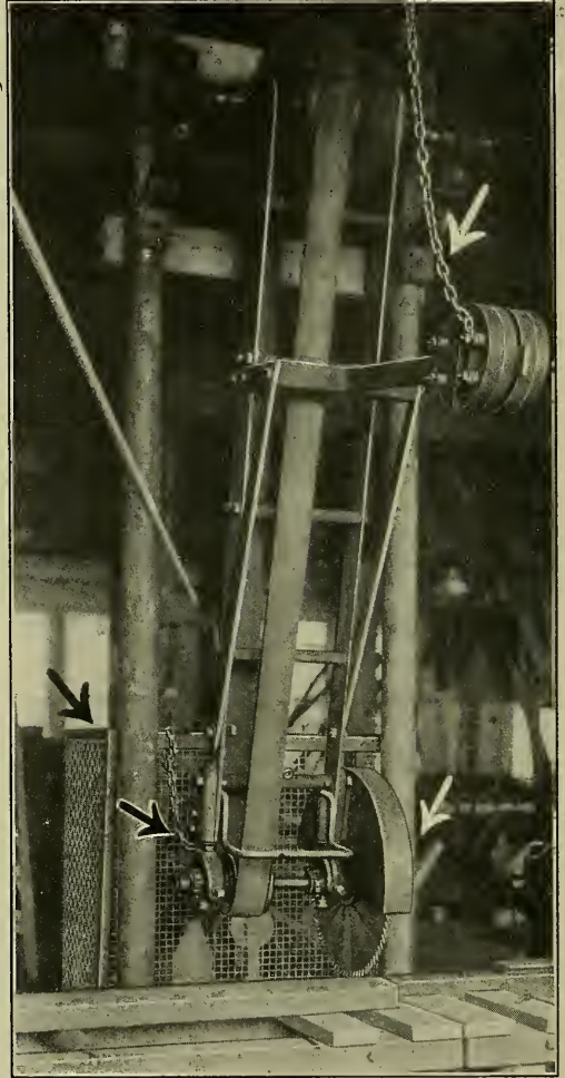
Fig. 132. Swing Saw Guards.
