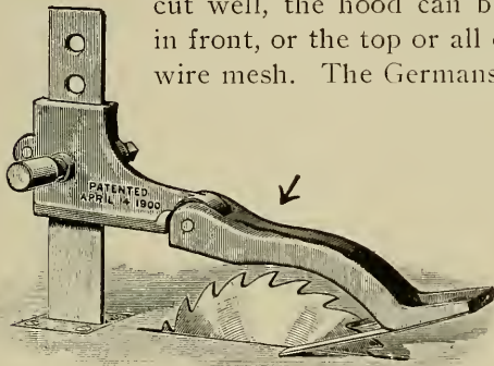
Fig. 90. Fay & Egan Saw Guard.
