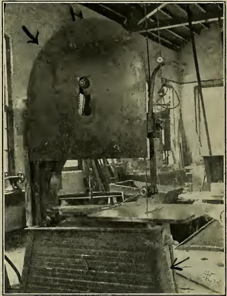
Courtesy of International Harvester Co. Fig. 140. Band Saw Guarded.
