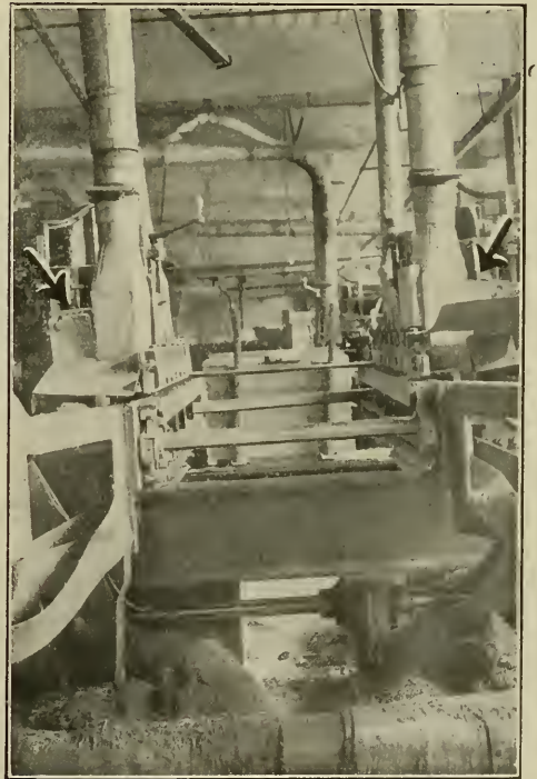
Fig. 214. Double End Tenoner Guarded, Rear View.
