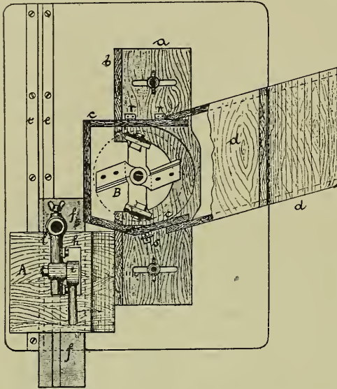
Fig. 170. Feeding Apparatus.
