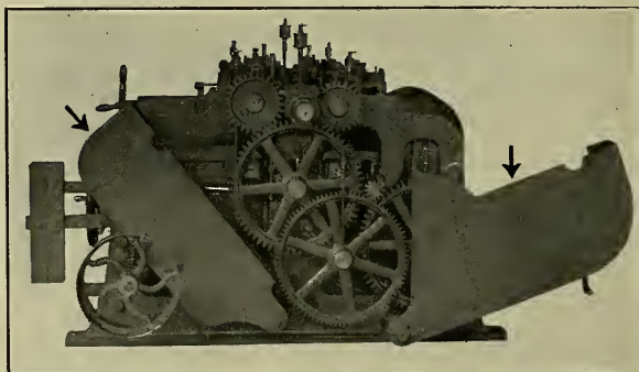
Fig. 203. Single Surfacers Guarded, Guards Open.
