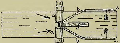
Fig. 162. Double Automatic Jointer Guard.
