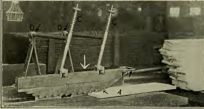
Fig. 102. Offutt Saw Guard, Raised by Material.
