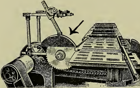
Fig. 118. Jones Railway Cut-Off Guard.
