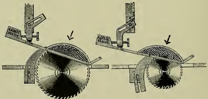
Fig. 99. Goede Saw Guard, Adjusted to Large and Small Saws.
