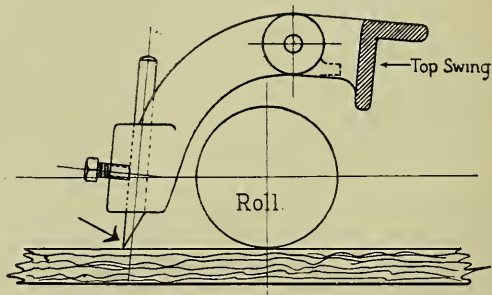
Fig. 20. Edger Dog Guard.
