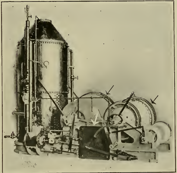
Fig. 4. Yarding Engine Guarded.
