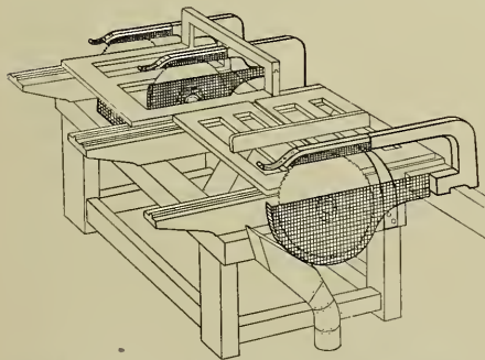
Fig. 277. Trimmer and Edger Guarded.
