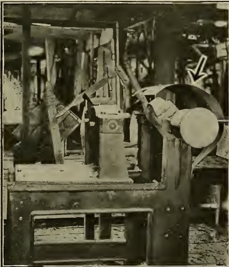
Fig. 281. Ladling Machine Guarded.
