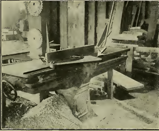
Fig. 161. Home-made Jointer Guard.
