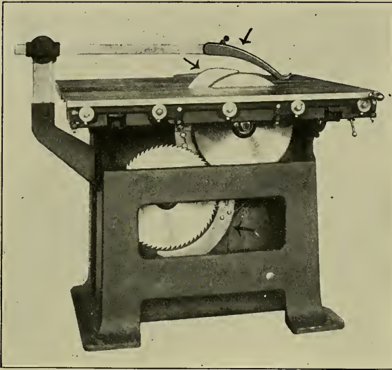
Fig. 265. Pattern-maker's Saws Guarded.
