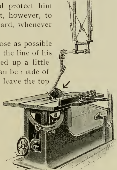
Fig. 91. Jones Saw Guard.
