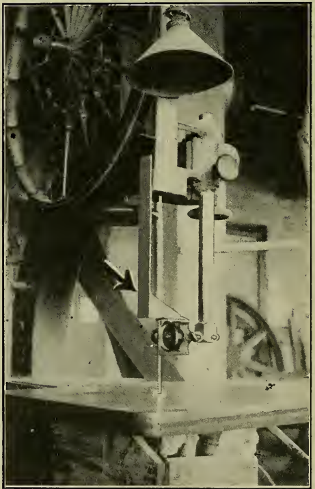
Courtesy of Link-Belt Co. Fig. 142. Guard for Band Saw Blade.
