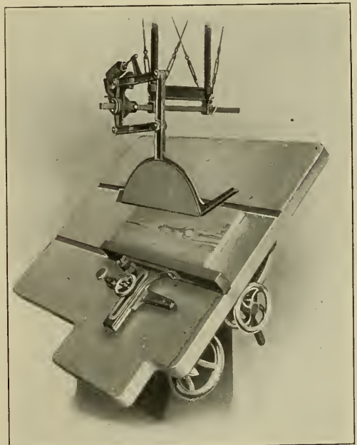
Fig. 108. Prybil Saw Guard.
