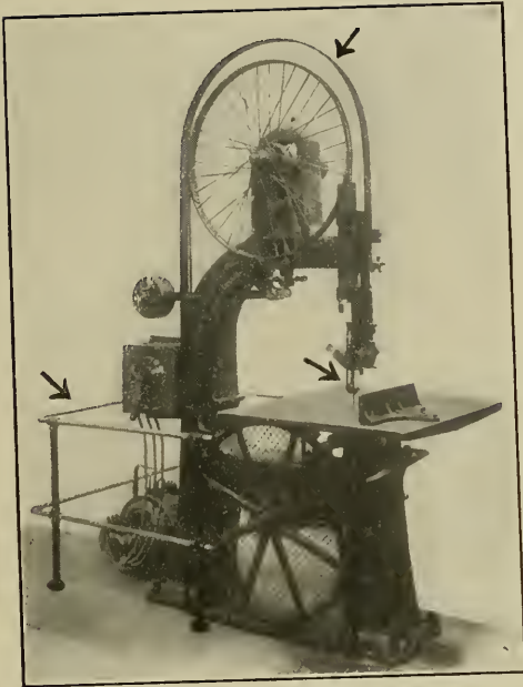
Fig. 143. German Guards for Band Saw.
