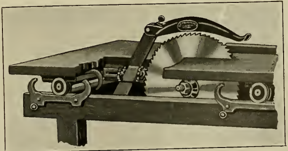
Fig. 87. Reliable Saw Guard.
