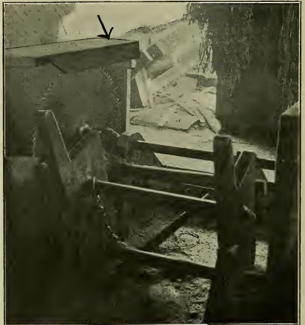
Fig. 66. Lath Trimmer Guarded.
