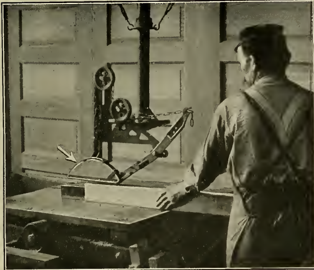
Fig. 107. Rockwell Saw Guard, 2 x 4 Being Ripped.
