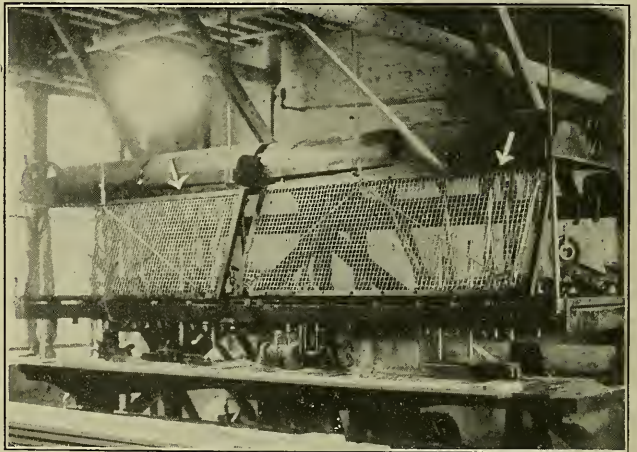
Fig. 207. Screen Guard for Multiple Boring Machine.
