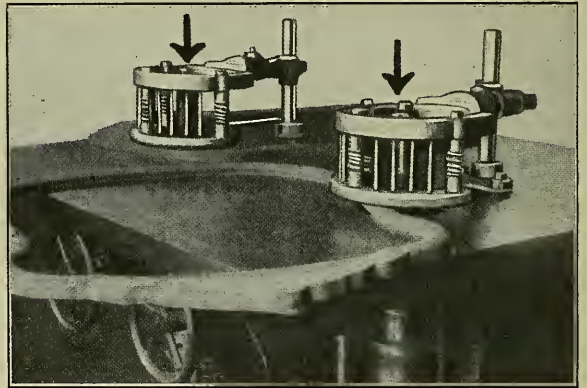
Fig. 181. Buckeye Shaper Guard.
