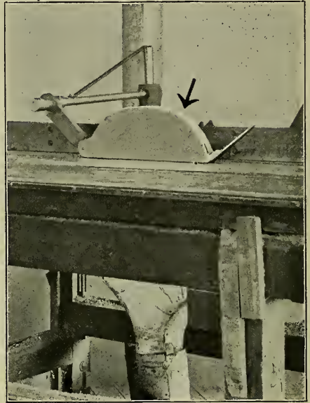
Courtesy of Fairbanks, Morse & Co. Fig. 110. McKee Saw Guard, Supported from Side of Table.
