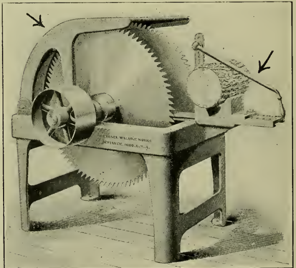
Fig. 128. Double Hub Equalizer Guarded.
