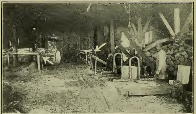
Fig. 124. Heading Bolter Saw Guarded.
