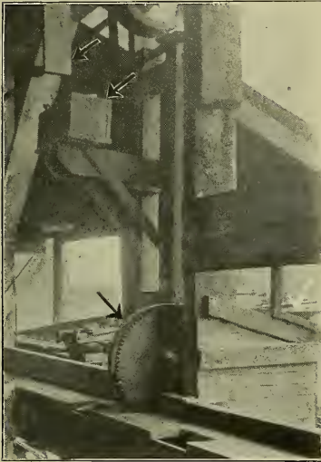
Fig. 32. Swing Trim Guarded.
