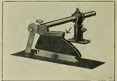
Fig. 98. Smith Saw Guard.
