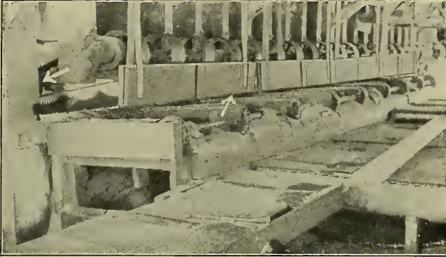
Fig. 29. Plank Guard Back of Overhead Trimmers.
