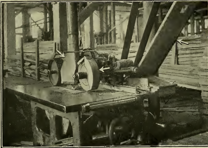
Fig. 114. Self-feed Rip Saw Guarded.
