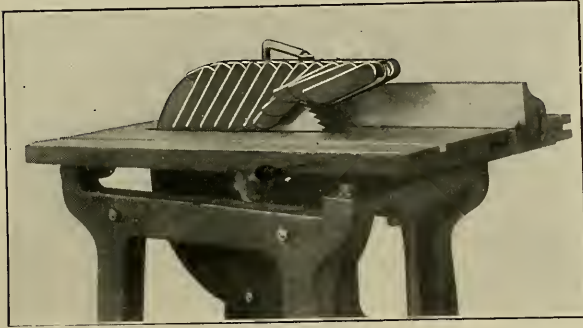
Fig. 104. German Finger Guard.
