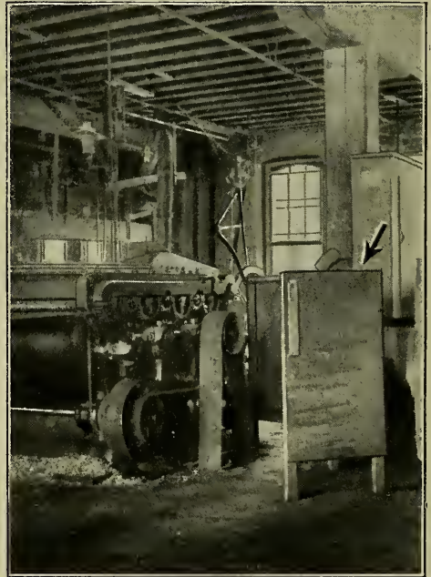
Courtesy of Widdicomb Furniture Co. Fig. 195. Sander Belt and Gear Housing Removed.
