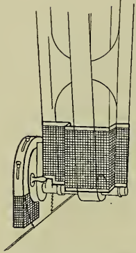
Fig. 135. Mesh Guards for Swing Saw.
