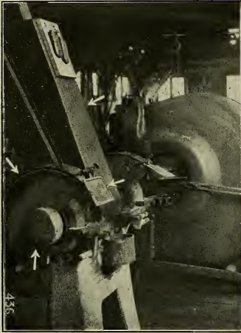
Fig. 311. Grinding Wheel Hoods, Eye Shields, Belt Guard and Arbor Cap.
