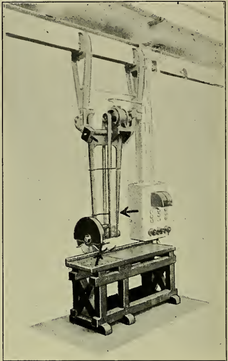
Fig. 136. German Swing Saw Guards.
