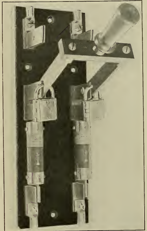
Fig. 305. Open Switch Padlocked.
