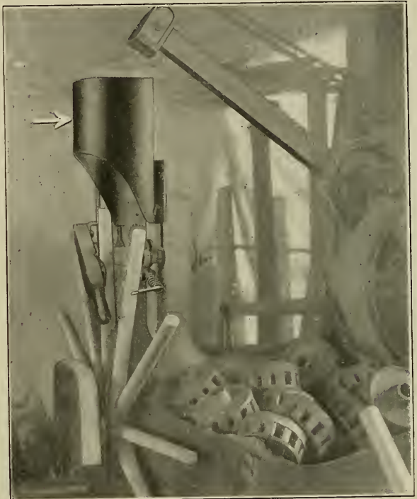
Fig. 233. Guard for Spoke Driver.
