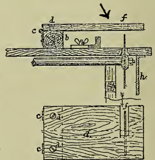
Courtesy of North German Woodworkers' Ass'n. Fig. 111. Guard for Grooving Saw.
