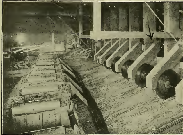
Fig. 39. Wooden Hoods for Slab Slashers.
