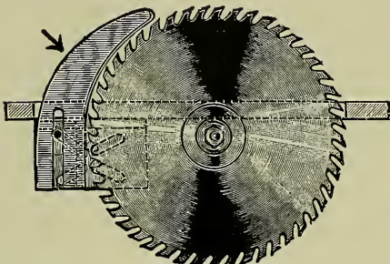
Fig. 83. Splitter Adjusted to Large Saw.
