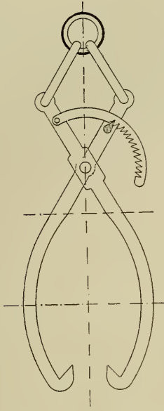
Fig. 55. Safety Tongs.
