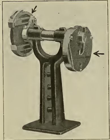
Fig. 313. Hood for Grinding Wheel.
