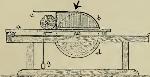
Fig. 120. Cut-Off Saw Guard.
