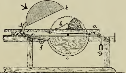
Fig. 121. Cut-Off Saw Guard.
