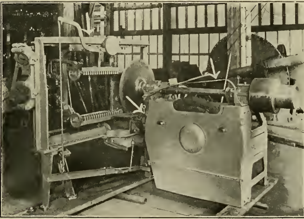
Fig. 70. Upright Shingle and Clip Saws.
