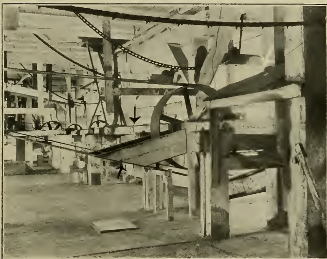
Fig. 48. Guarded Transmission.
