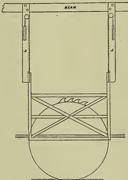
Fig. 221. Guard for Short Log Saw Mill.
