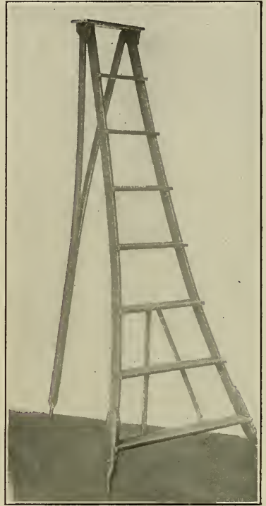
Courtesy of International Harvester Co. Fig. 307. Safety Oiler's Ladder.
