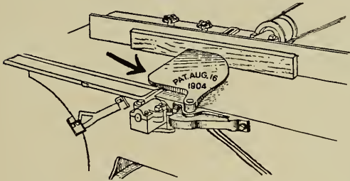
Fig. 155. Badger Jointer Guard.
