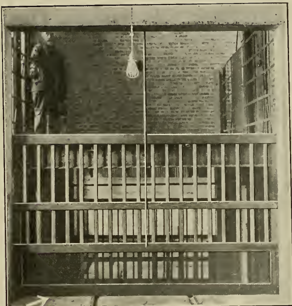
Fig. 317. Elevator Gate Screened at Bottom.
