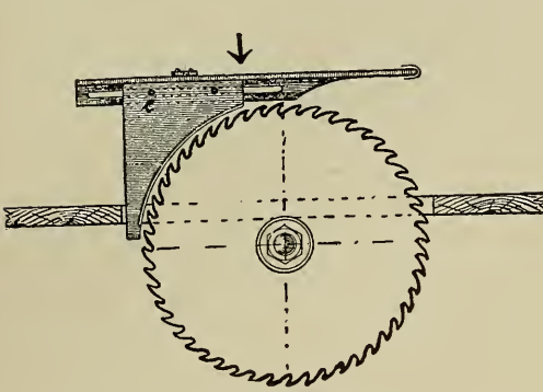
Fig. 85. Splitter Supported from Above.
