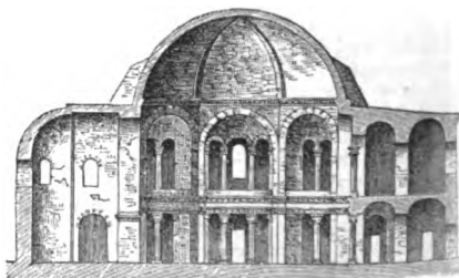
No. 3. Section of the Church of SS. Sergius and Basilius, Constantinople.
